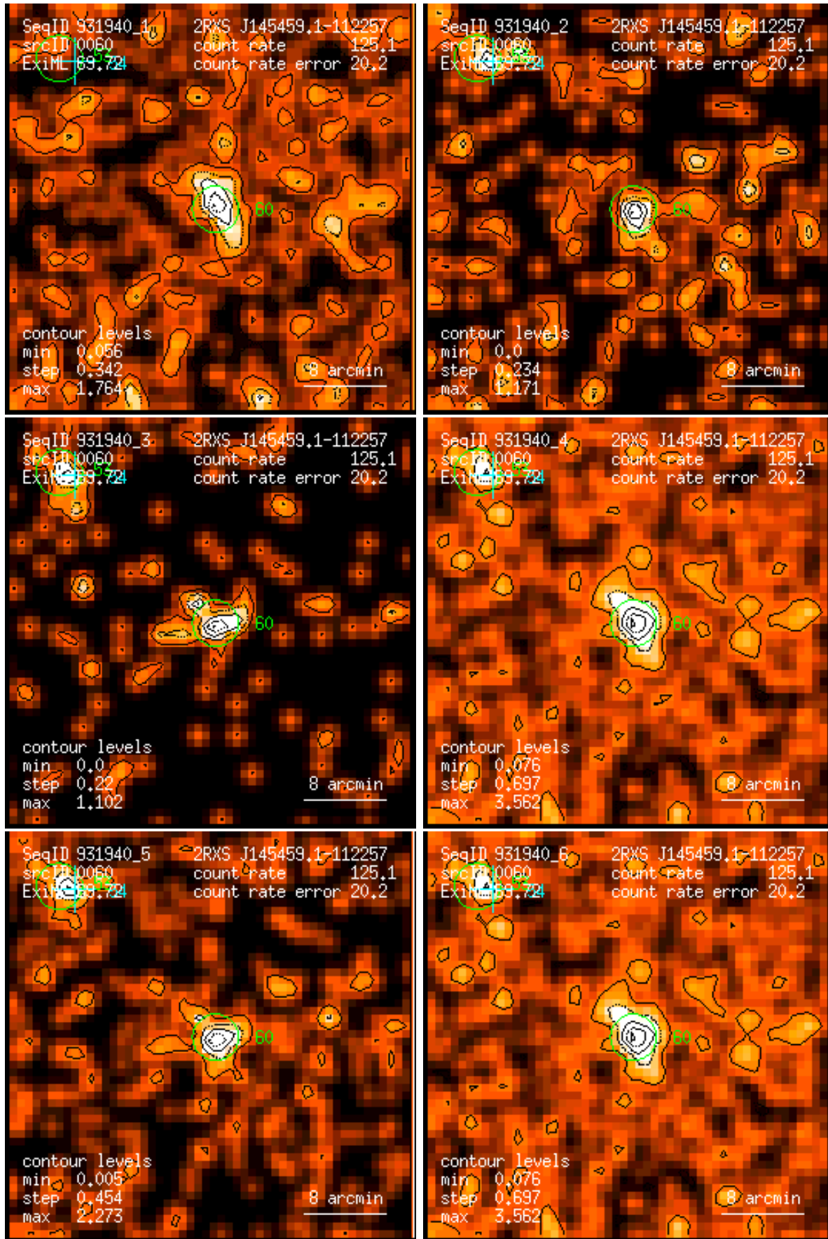
Figure 60: RASS 931940: detection 0060: band rate images, Gaussian filter: (1) PSPC channels 11 – 41, (2) 52 – 90, (3) 91 – 201, (4) 11 – 235, (5) 52 – 201, (6) 11 – 201. Broad band rates in counts/ks. Band rate contour levels in counts/ks/arcmin 2 .
