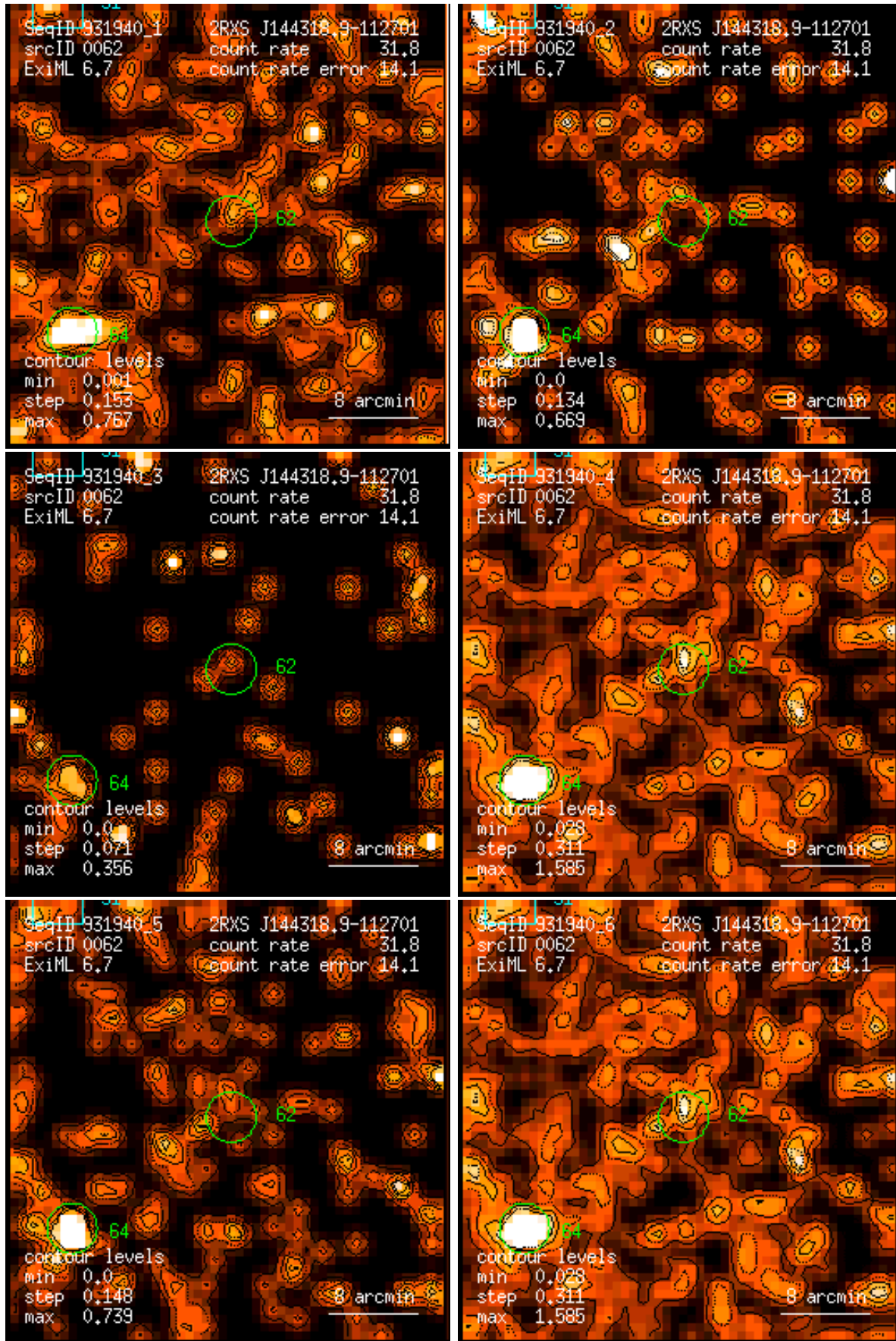
Figure 62: RASS 931940: detection 0062: band rate images, Gaussian filter: (1) PSPC channels 11 – 41, (2) 52 – 90, (3) 91 – 201, (4) 11 – 235, (5) 52 – 201, (6) 11 – 201. Broad band rates in counts/ks. Band rate contour levels in counts/ks/arcmin 2 .
