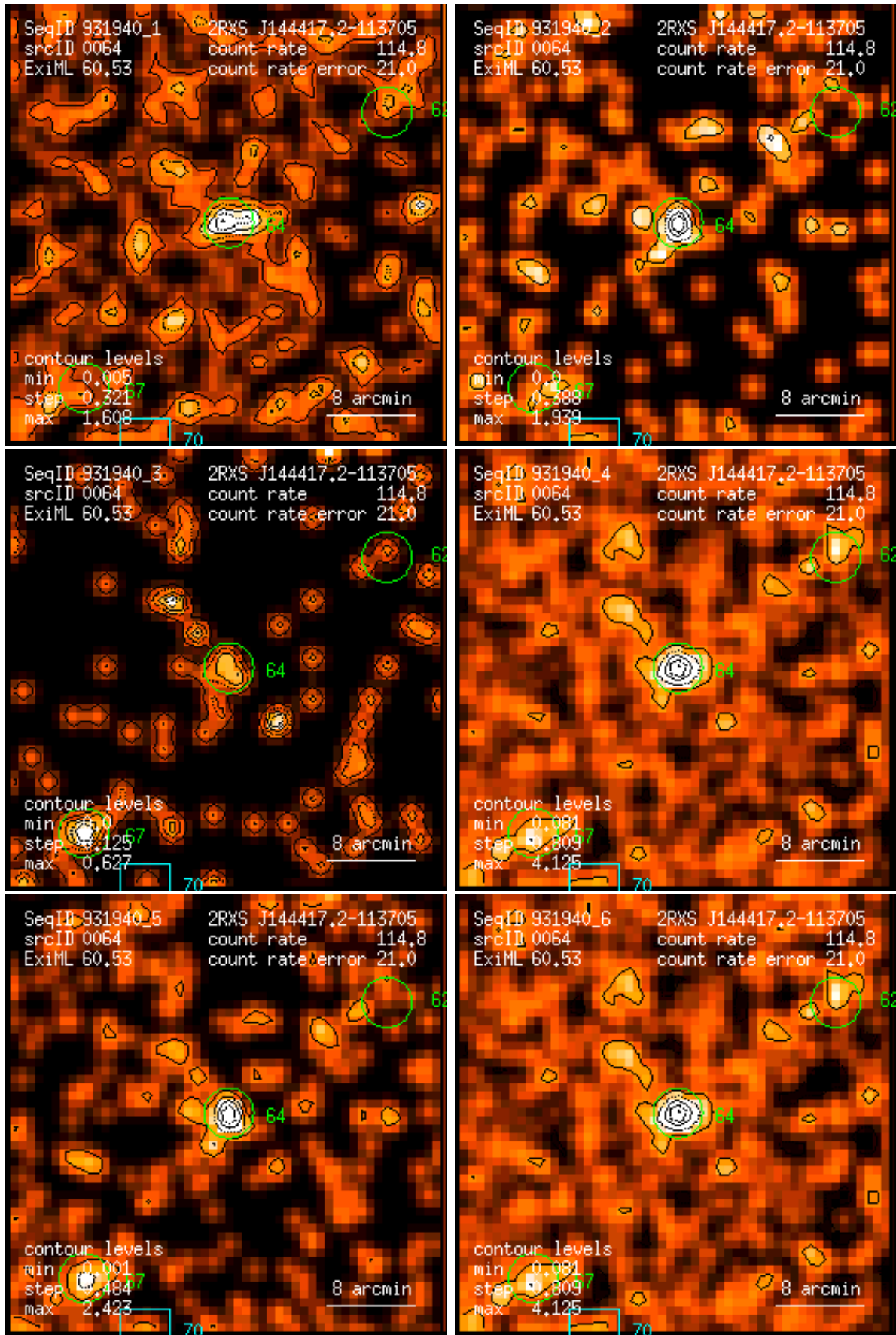
Figure 64: RASS 931940: detection 0064: band rate images, Gaussian filter: (1) PSPC channels 11 – 41, (2) 52 – 90, (3) 91 – 201, (4) 11 – 235, (5) 52 – 201, (6) 11 – 201. Broad band rates in counts/ks. Band rate contour levels in counts/ks/arcmin 2 .
