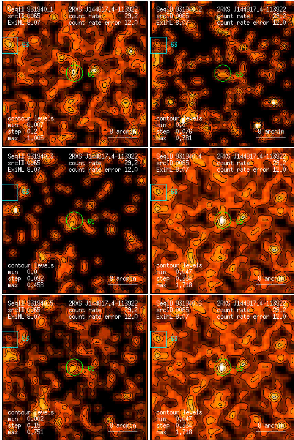
Figure 65: RASS 931940: detection 0065: band rate images, Gaussian filter: (1) PSPC channels 11 – 41, (2) 52 – 90, (3) 91 – 201, (4) 11 – 235, (5) 52 – 201, (6) 11 – 201. Broad band rates in counts/ks. Band rate contour levels in counts/ks/arcmin 2 .
