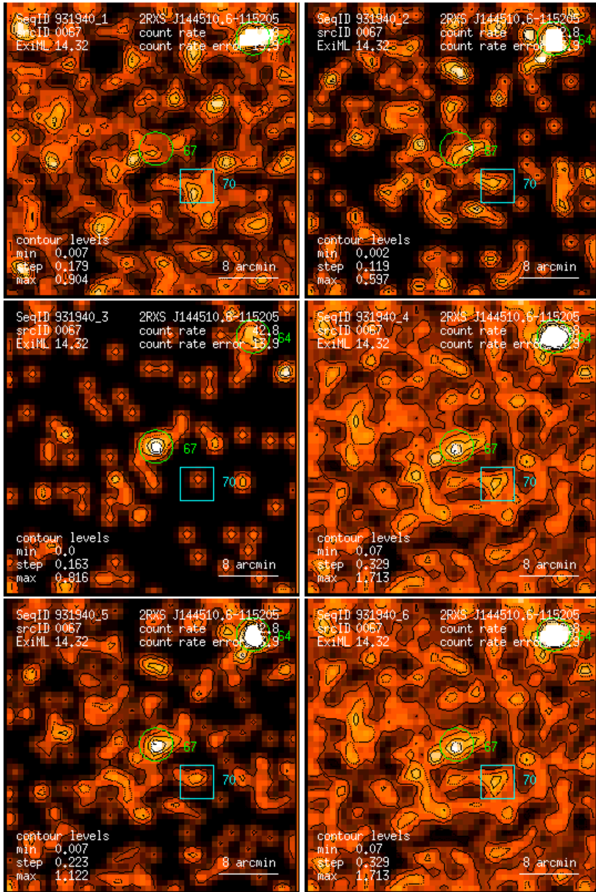
Figure 67: RASS 931940: detection 0067: band rate images, Gaussian filter: (1) PSPC channels 11 – 41, (2) 52 – 90, (3) 91 – 201, (4) 11 – 235, (5) 52 – 201, (6) 11 – 201. Broad band rates in counts/ks. Band rate contour levels in counts/ks/arcmin 2 .
