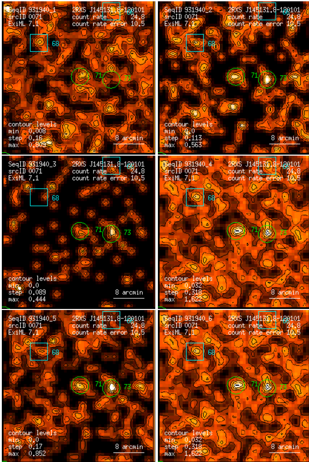
Figure 71: RASS 931940: detection 0071: band rate images, Gaussian filter: (1) PSPC channels 11 – 41, (2) 52 – 90, (3) 91 – 201, (4) 11 – 235, (5) 52 – 201, (6) 11 – 201. Broad band rates in counts/ks. Band rate contour levels in counts/ks/arcmin 2 .
