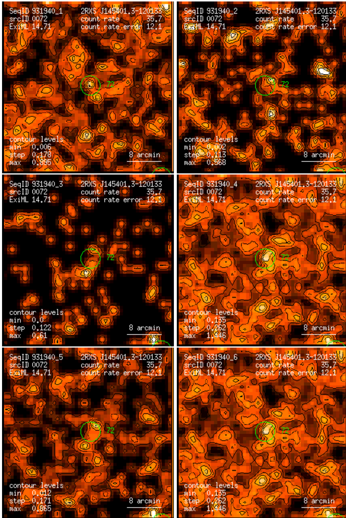
Figure 72: RASS 931940: detection 0072: band rate images, Gaussian filter: (1) PSPC channels 11 – 41, (2) 52 – 90, (3) 91 – 201, (4) 11 – 235, (5) 52 – 201, (6) 11 – 201. Broad band rates in counts/ks. Band rate contour levels in counts/ks/arcmin 2 .
