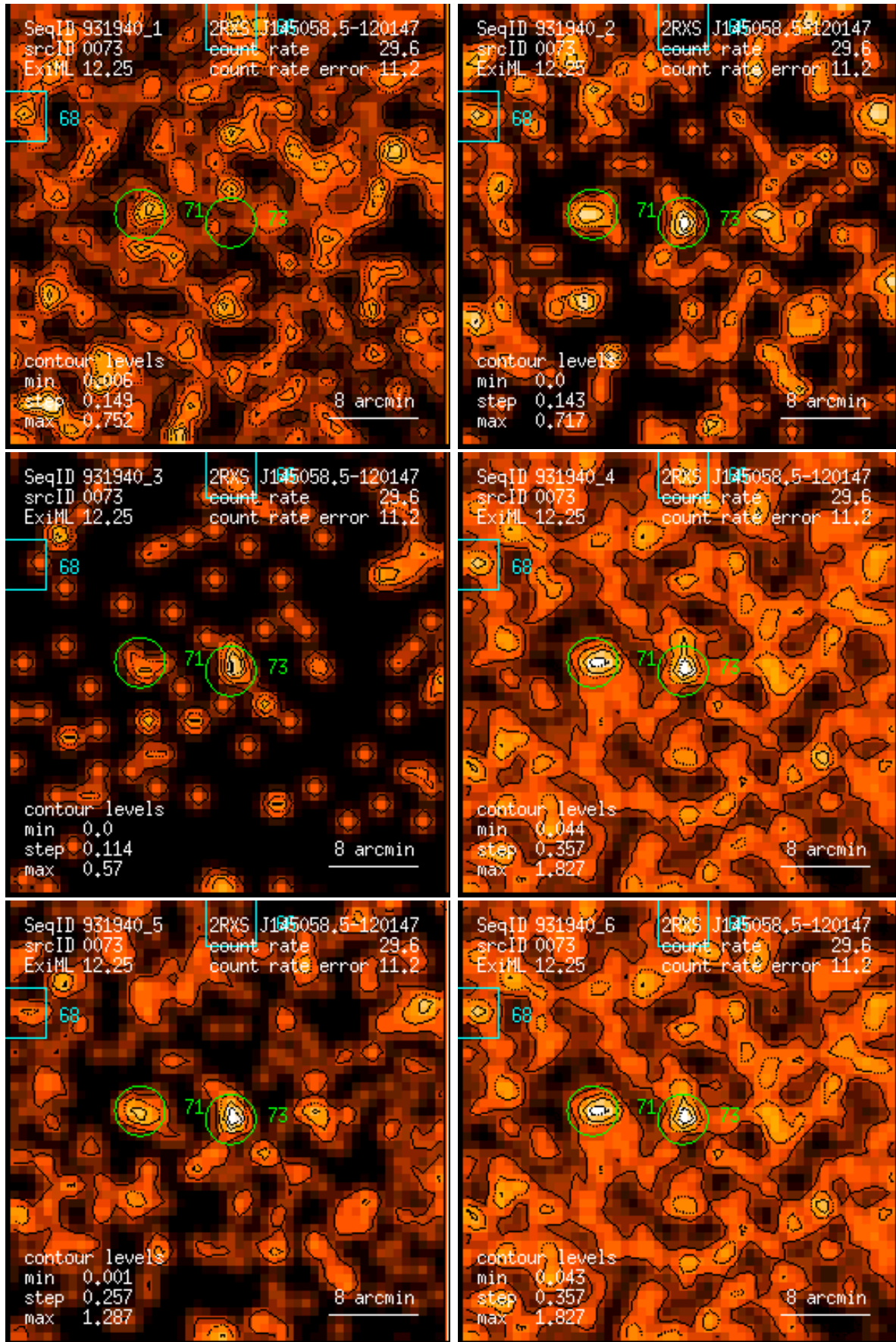
Figure 73: RASS 931940: detection 0073: band rate images, Gaussian filter: (1) PSPC channels 11 – 41, (2) 52 – 90, (3) 91 – 201, (4) 11 – 235, (5) 52 – 201, (6) 11 – 201. Broad band rates in counts/ks. Band rate contour levels in counts/ks/arcmin 2 .
