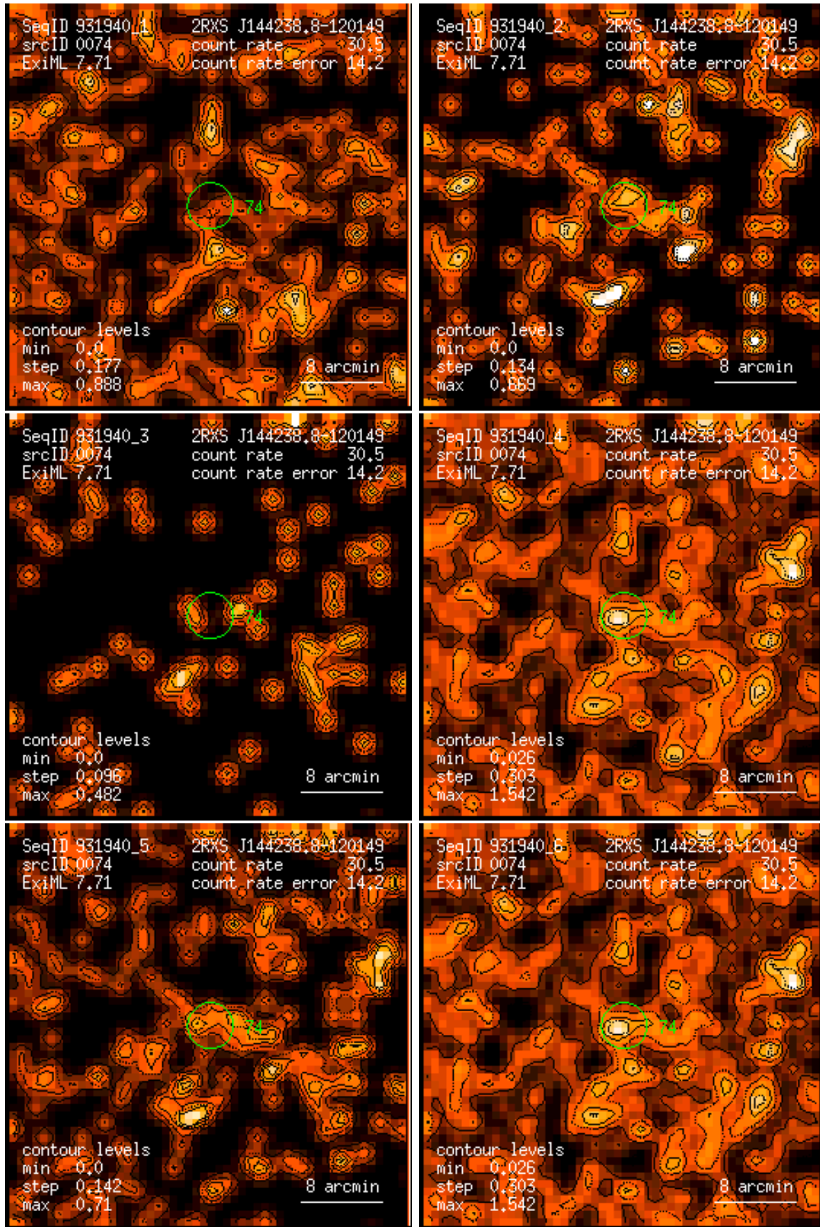
Figure 74: RASS 931940: detection 0074: band rate images, Gaussian filter: (1) PSPC channels 11 – 41, (2) 52 – 90, (3) 91 – 201, (4) 11 – 235, (5) 52 – 201, (6) 11 – 201. Broad band rates in counts/ks. Band rate contour levels in counts/ks/arcmin 2 .
