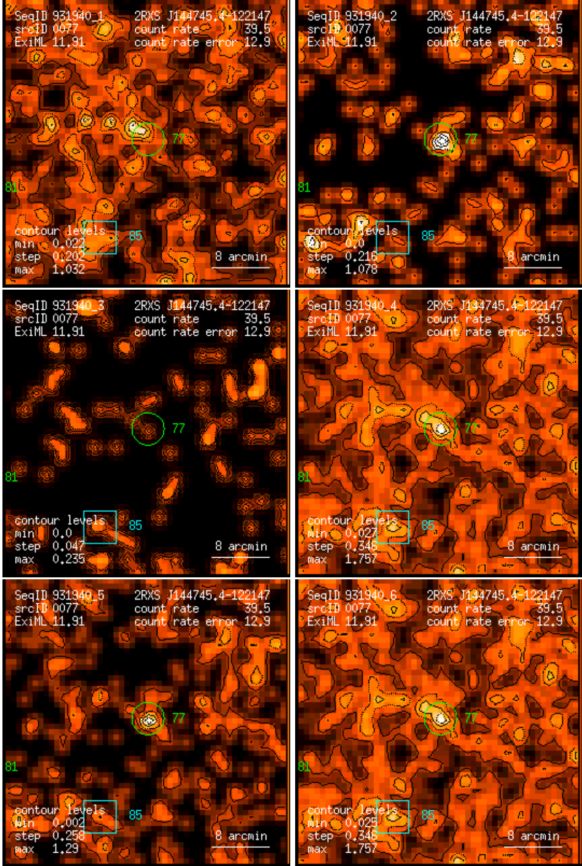
Figure 77: RASS 931940: detection 0077: band rate images, Gaussian filter: (1) PSPC channels 11 – 41, (2) 52 – 90, (3) 91 – 201, (4) 11 – 235, (5) 52 – 201, (6) 11 – 201. Broad band rates in counts/ks. Band rate contour levels in counts/ks/arcmin 2 .
