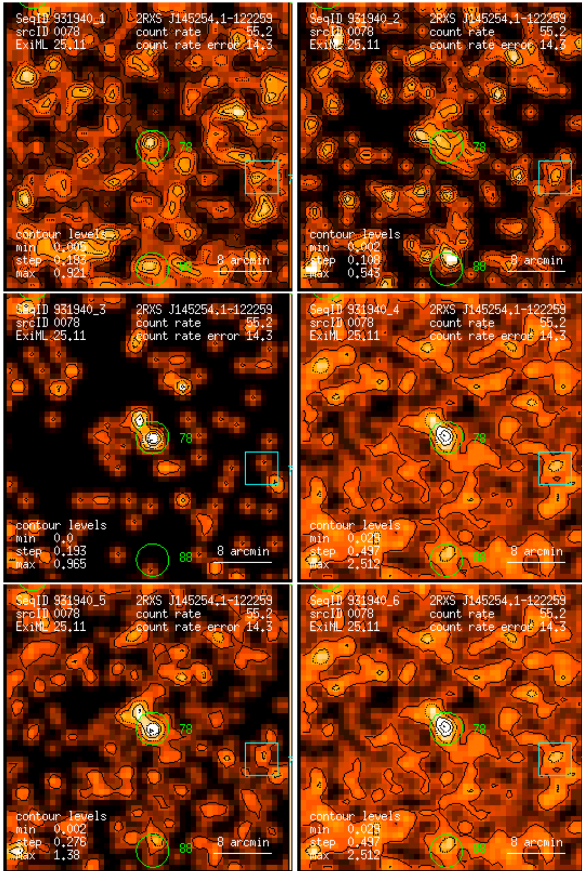
Figure 78: RASS 931940: detection 0078: band rate images, Gaussian filter: (1) PSPC channels 11 – 41, (2) 52 – 90, (3) 91 – 201, (4) 11 – 235, (5) 52 – 201, (6) 11 – 201. Broad band rates in counts/ks. Band rate contour levels in counts/ks/arcmin 2 .
