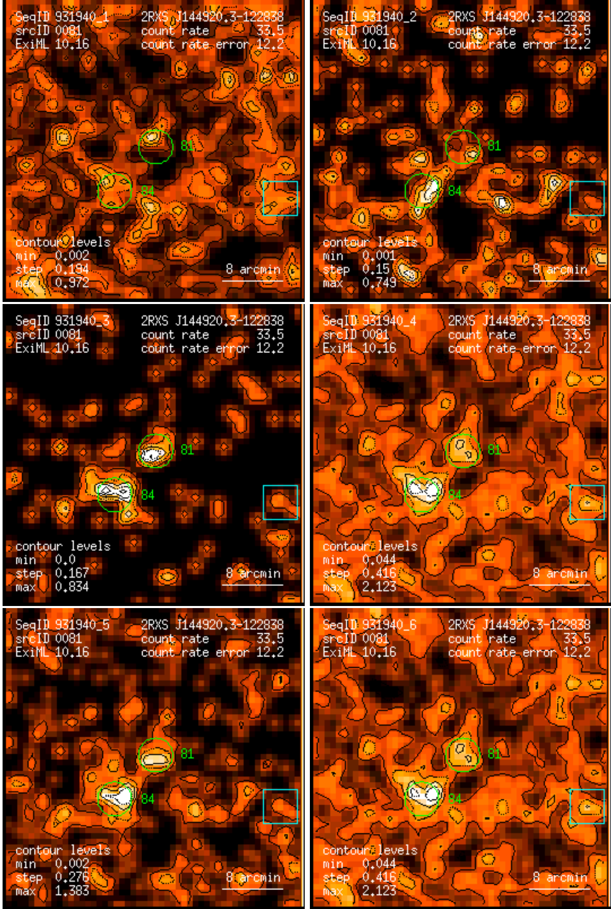
Figure 81: RASS 931940: detection 0081: band rate images, Gaussian filter: (1) PSPC channels 11 – 41, (2) 52 – 90, (3) 91 – 201, (4) 11 – 235, (5) 52 – 201, (6) 11 – 201. Broad band rates in counts/ks. Band rate contour levels in counts/ks/arcmin 2 .
