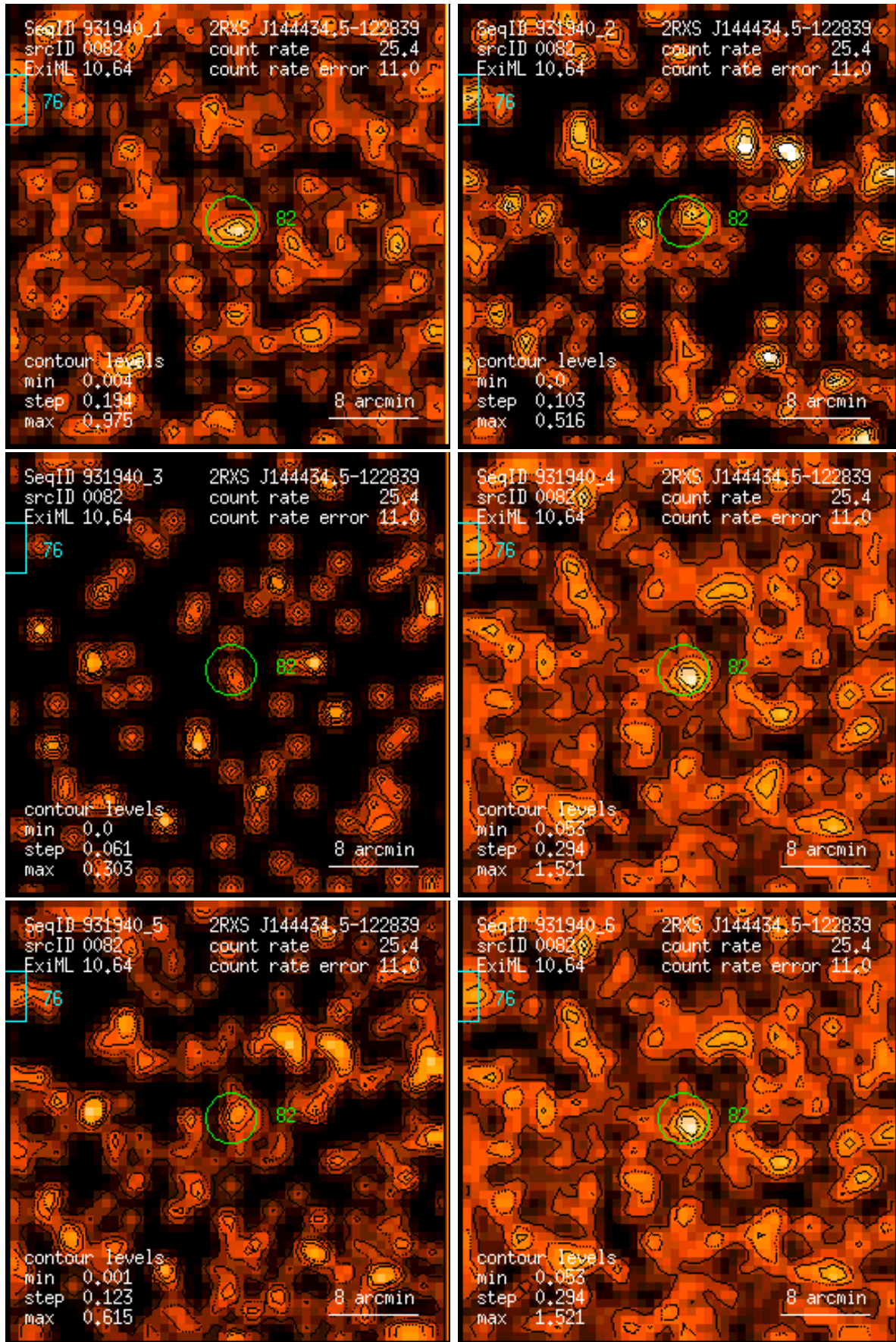
Figure 82: RASS 931940: detection 0082: band rate images, Gaussian filter: (1) PSPC channels 11 – 41, (2) 52 – 90, (3) 91 – 201, (4) 11 – 235, (5) 52 – 201, (6) 11 – 201. Broad band rates in counts/ks. Band rate contour levels in counts/ks/arcmin 2 .
