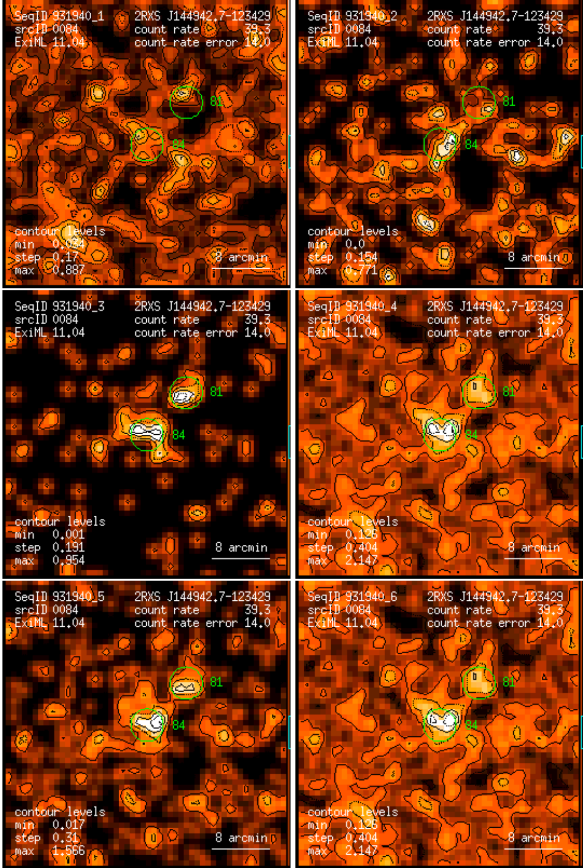
Figure 84: RASS 931940: detection 0084: band rate images, Gaussian filter: (1) PSPC channels 11 – 41, (2) 52 – 90, (3) 91 – 201, (4) 11 – 235, (5) 52 – 201, (6) 11 – 201. Broad band rates in counts/ks. Band rate contour levels in counts/ks/arcmin 2 .
