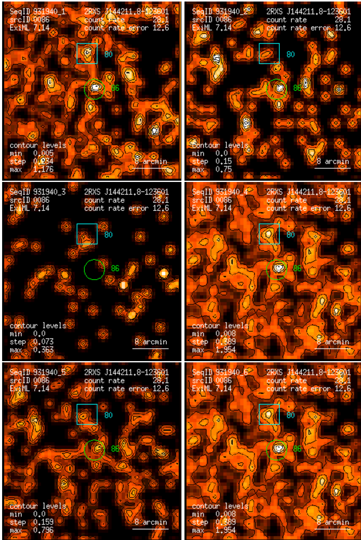
Figure 86: RASS 931940: detection 0086: band rate images, Gaussian filter: (1) PSPC channels 11 – 41, (2) 52 – 90, (3) 91 – 201, (4) 11 – 235, (5) 52 – 201, (6) 11 – 201. Broad band rates in counts/ks. Band rate contour levels in counts/ks/arcmin 2 .
