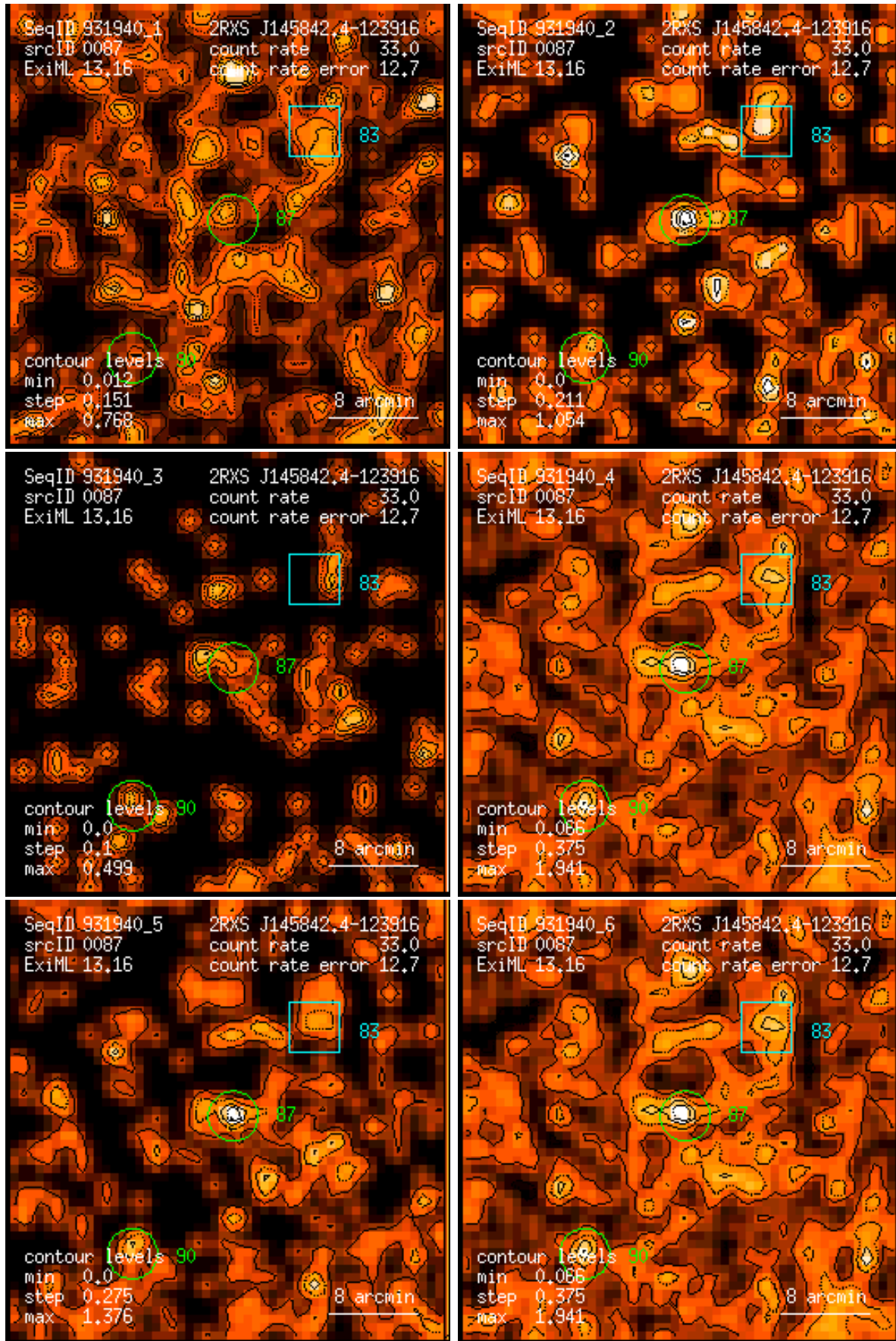
Figure 87: RASS 931940: detection 0087: band rate images, Gaussian filter: (1) PSPC channels 11 – 41, (2) 52 – 90, (3) 91 – 201, (4) 11 – 235, (5) 52 – 201, (6) 11 – 201. Broad band rates in counts/ks. Band rate contour levels in counts/ks/arcmin 2 .
