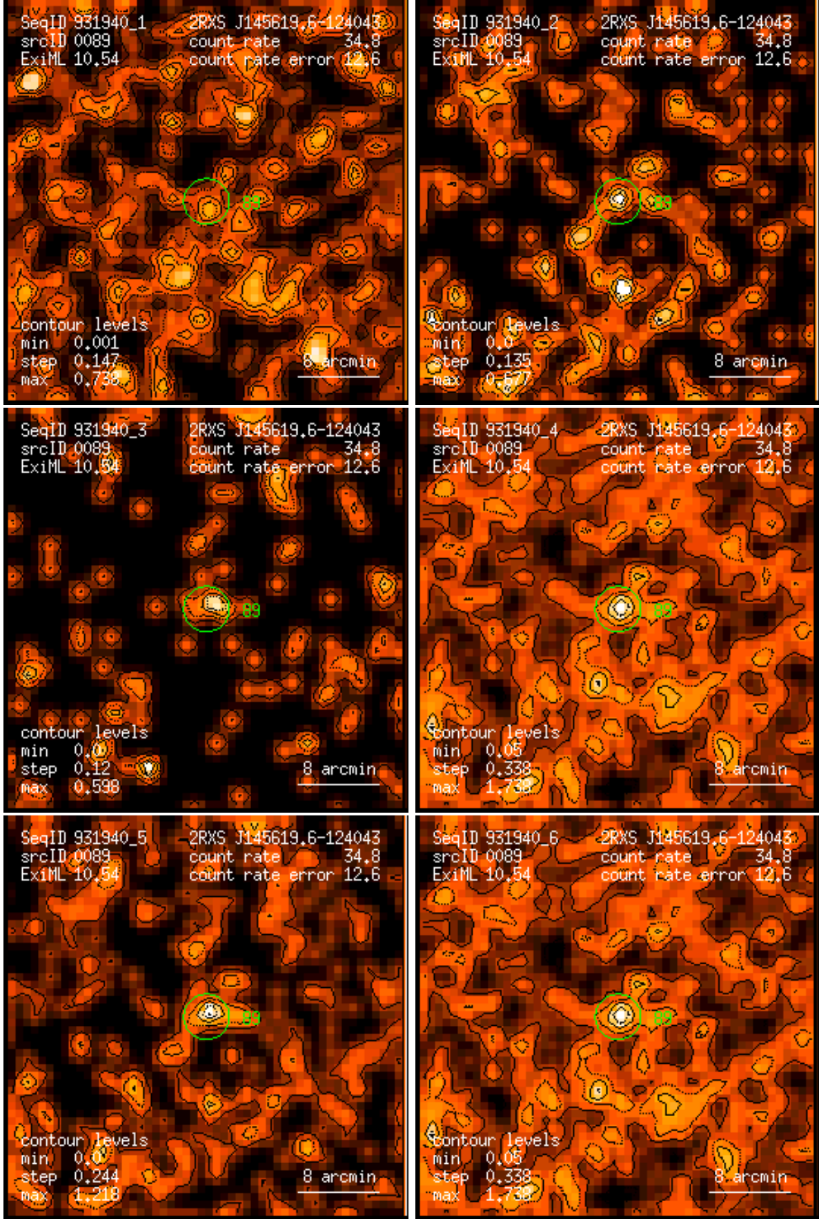
Figure 89: RASS 931940: detection 0089: band rate images, Gaussian filter: (1) PSPC channels 11 – 41, (2) 52 – 90, (3) 91 – 201, (4) 11 – 235, (5) 52 – 201, (6) 11 – 201. Broad band rates in counts/ks. Band rate contour levels in counts/ks/arcmin 2 .
