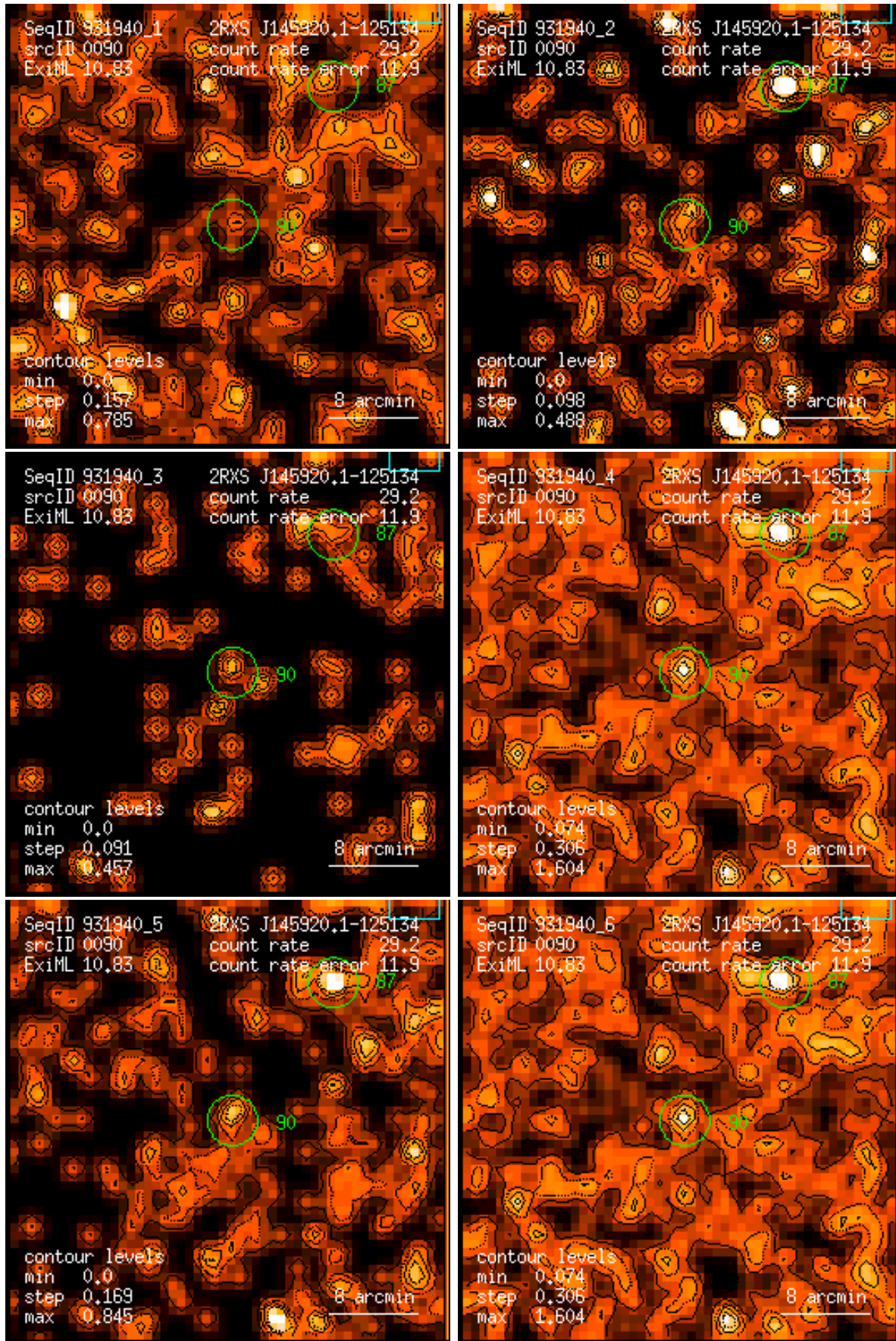
Figure 90: RASS 931940: detection 0090: band rate images, Gaussian filter: (1) PSPC channels 11 – 41, (2) 52 – 90, (3) 91 – 201, (4) 11 – 235, (5) 52 – 201, (6) 11 – 201. Broad band rates in counts/ks. Band rate contour levels in counts/ks/arcmin 2 .
