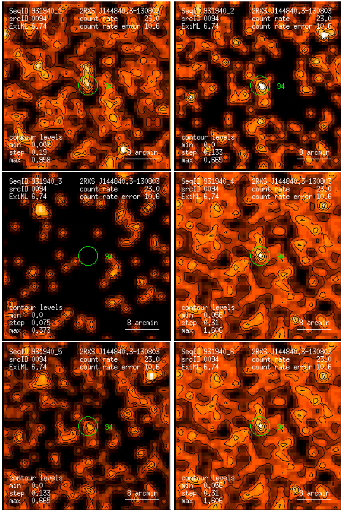
Figure 94: RASS 931940: detection 0094: band rate images, Gaussian filter: (1) PSPC channels 11 – 41, (2) 52 – 90, (3) 91 – 201, (4) 11 – 235, (5) 52 – 201, (6) 11 – 201. Broad band rates in counts/ks. Band rate contour levels in counts/ks/arcmin 2 .
