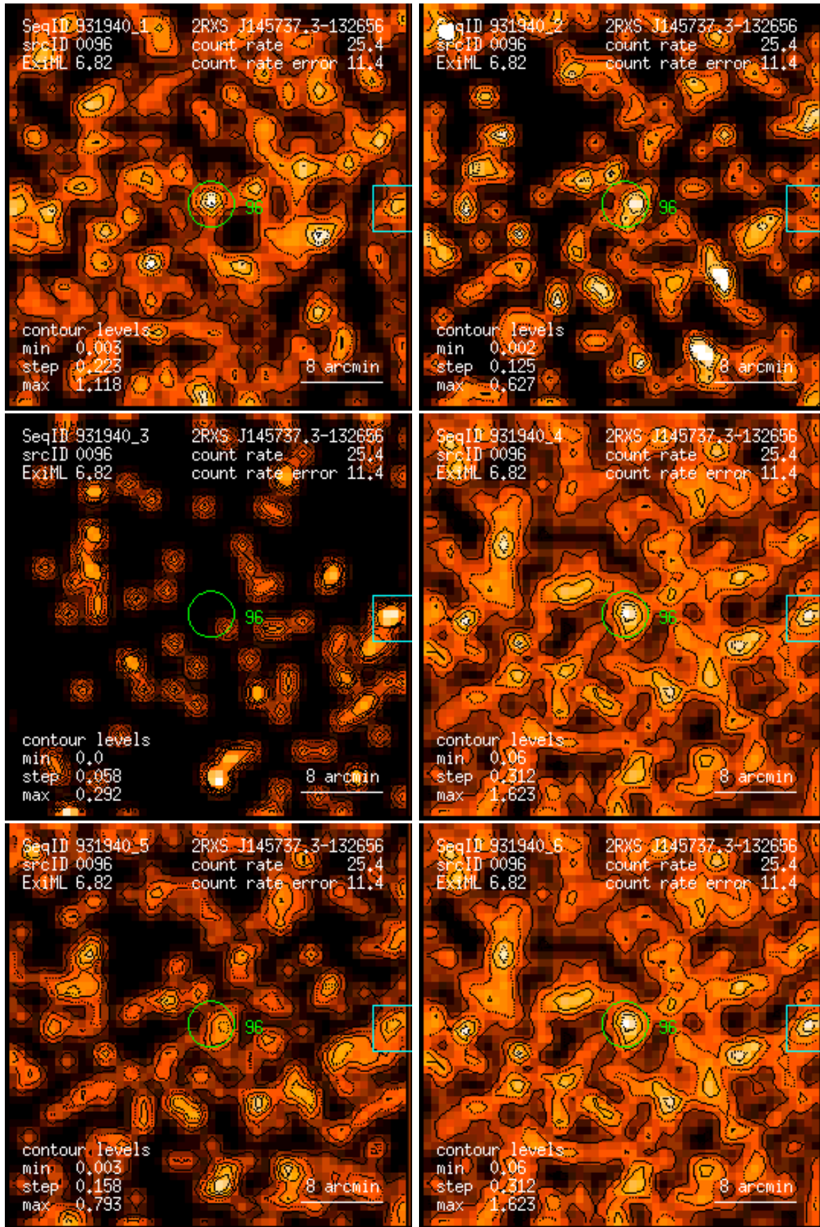
Figure 96: RASS 931940: detection 0096: band rate images, Gaussian filter: (1) PSPC channels 11 – 41, (2) 52 – 90, (3) 91 – 201, (4) 11 – 235, (5) 52 – 201, (6) 11 – 201. Broad band rates in counts/ks. Band rate contour levels in counts/ks/arcmin 2 .
