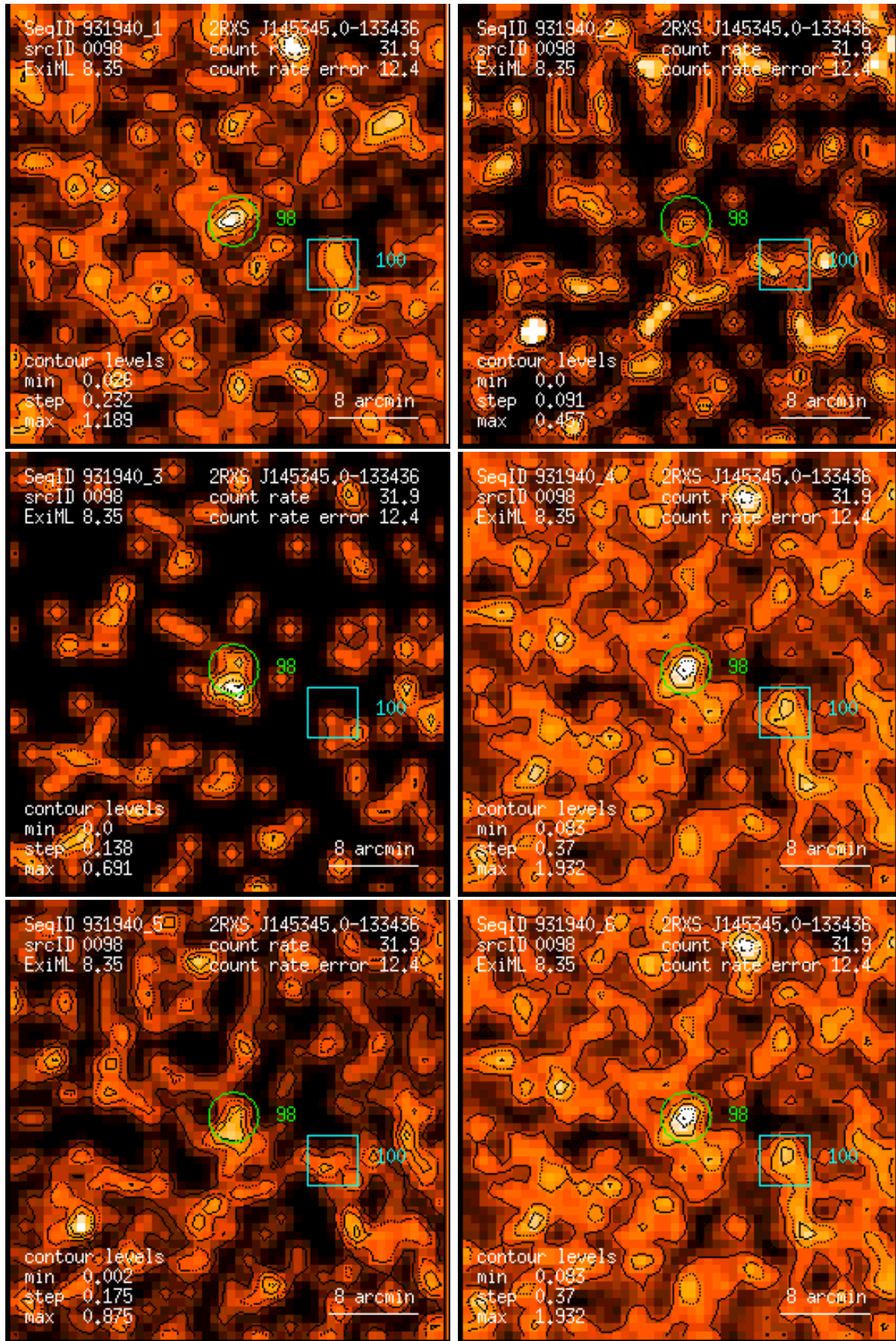
Figure 98: RASS 931940: detection 0098: band rate images, Gaussian filter: (1) PSPC channels 11 – 41, (2) 52 – 90, (3) 91 – 201, (4) 11 – 235, (5) 52 – 201, (6) 11 – 201. Broad band rates in counts/ks. Band rate contour levels in counts/ks/arcmin 2 .
