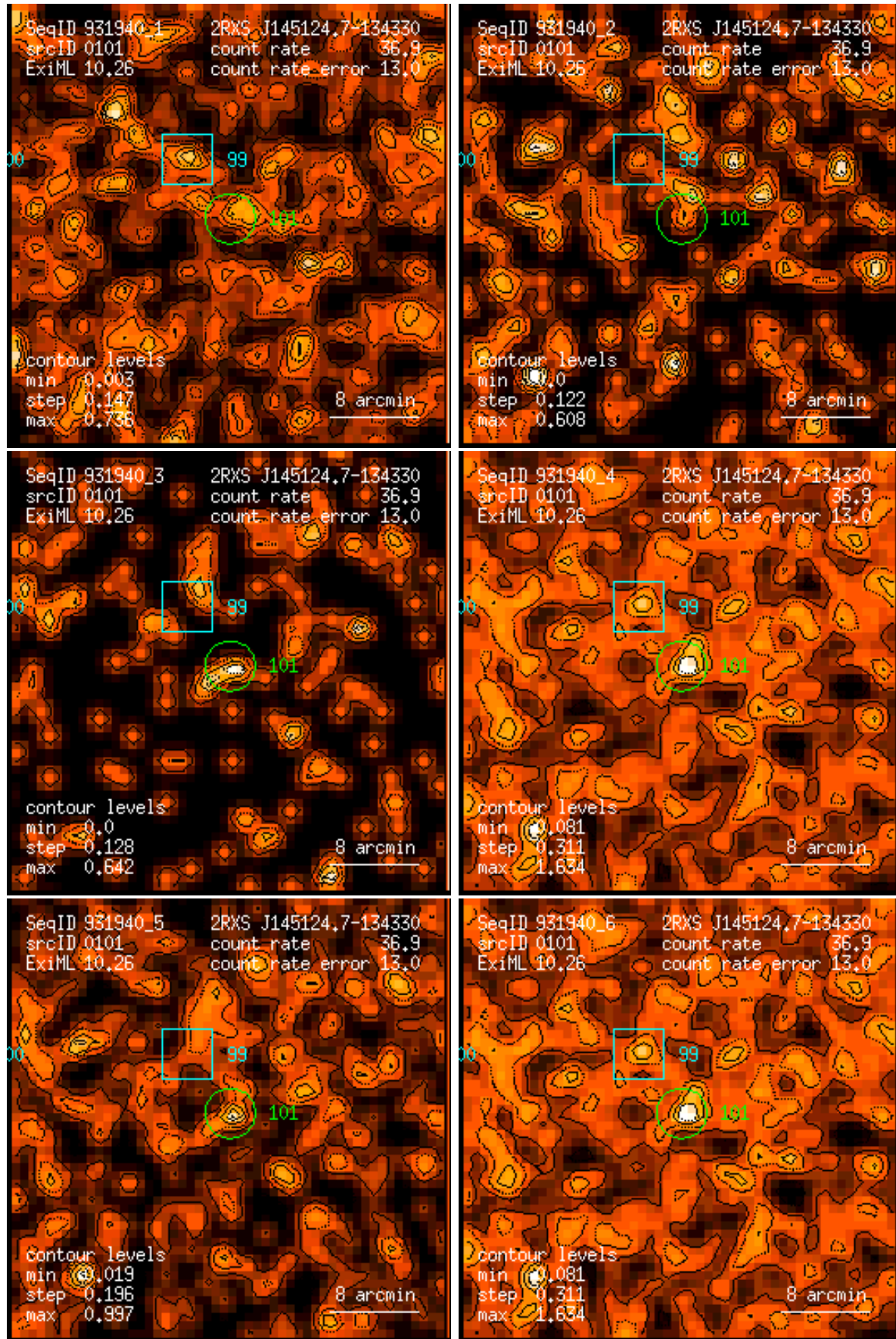
Figure 101: RASS 931940: detection 0101: band rate images, Gaussian filter: (1) PSPC channels 11 – 41, (2) 52 – 90, (3) 91 – 201, (4) 11 – 235, (5) 52 – 201, (6) 11 – 201. Broad band rates in counts/ks. Band rate contour levels in counts/ks/arcmin 2 .
