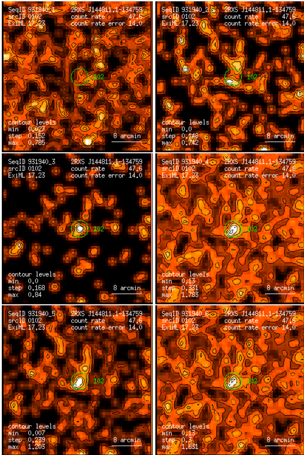
Figure 102: RASS 931940: detection 0102: band rate images, Gaussian filter: (1) PSPC channels 11 – 41, (2) 52 – 90, (3) 91 – 201, (4) 11 – 235, (5) 52 – 201, (6) 11 – 201. Broad band rates in counts/ks. Band rate contour levels in counts/ks/arcmin 2 .
