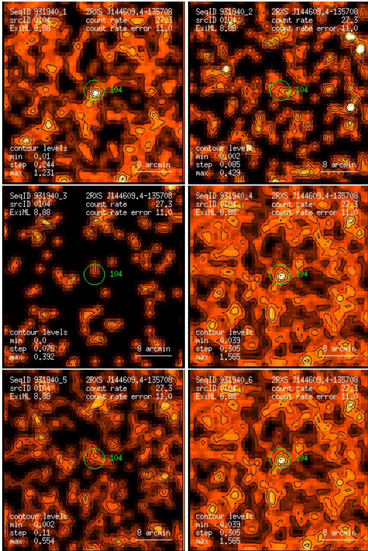
Figure 104: RASS 931940: detection 0104: band rate images, Gaussian filter: (1) PSPC channels 11 – 41, (2) 52 – 90, (3) 91 – 201, (4) 11 – 235, (5) 52 – 201, (6) 11 – 201. Broad band rates in counts/ks. Band rate contour levels in counts/ks/arcmin 2 .
