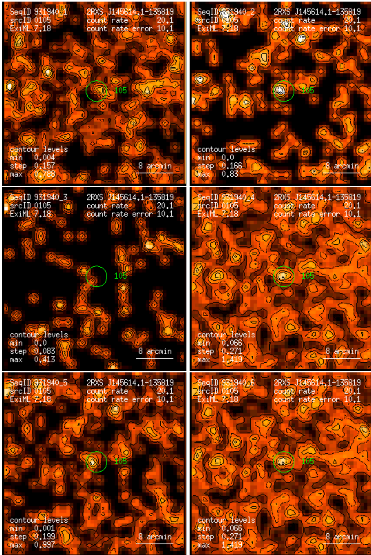
Figure 105: RASS 931940: detection 0105: band rate images, Gaussian filter: (1) PSPC channels 11 – 41, (2) 52 – 90, (3) 91 – 201, (4) 11 – 235, (5) 52 – 201, (6) 11 – 201. Broad band rates in counts/ks. Band rate contour levels in counts/ks/arcmin 2 .
