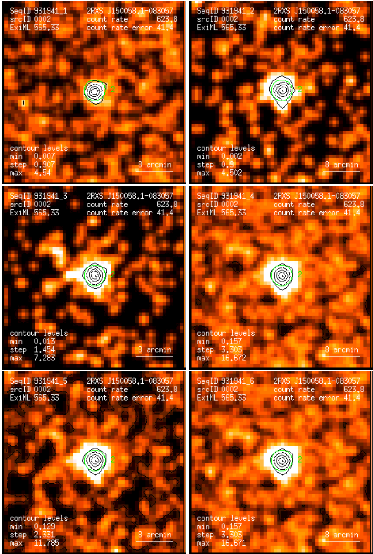
Figure 2: RASS 931941: detection 0002: band rate images, Gaussian filter: (1) PSPC channels 11 – 41, (2) 52 – 90, (3) 91 – 201, (4) 11 – 235, (5) 52 – 201, (6) 11 – 201. Broad band rates in counts/ks. Band rate contour levels in counts/ks/arcmin 2 .
