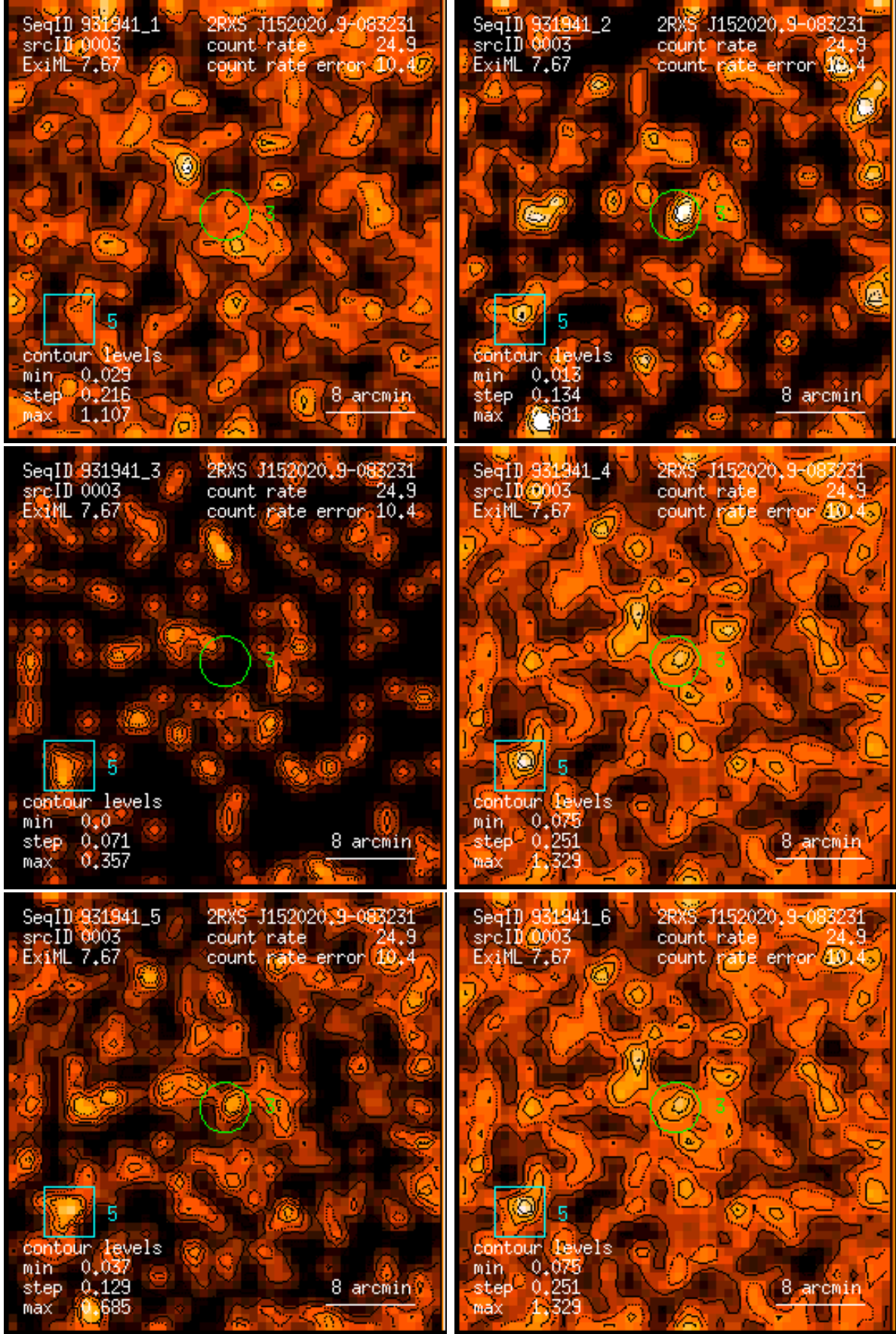
Figure 3: RASS 931941: detection 0003: band rate images, Gaussian filter: (1) PSPC channels 11 – 41, (2) 52 – 90, (3) 91 – 201, (4) 11 – 235, (5) 52 – 201, (6) 11 – 201. Broad band rates in counts/ks. Band rate contour levels in counts/ks/arcmin 2 .
