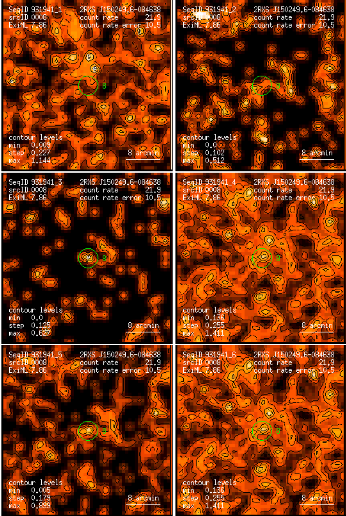
Figure 8: RASS 931941: detection 0008: band rate images, Gaussian filter: (1) PSPC channels 11 – 41, (2) 52 – 90, (3) 91 – 201, (4) 11 – 235, (5) 52 – 201, (6) 11 – 201. Broad band rates in counts/ks. Band rate contour levels in counts/ks/arcmin 2 .
