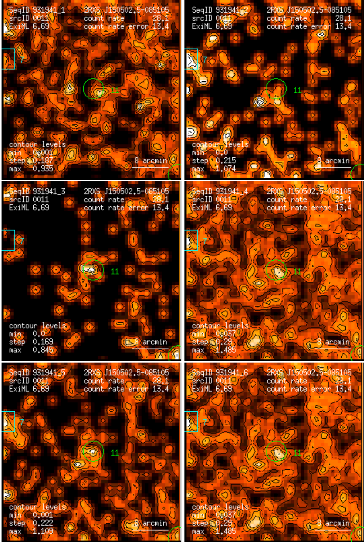
Figure 11: RASS 931941: detection 0011: band rate images, Gaussian filter: (1) PSPC channels 11 – 41, (2) 52 – 90, (3) 91 – 201, (4) 11 – 235, (5) 52 – 201, (6) 11 – 201. Broad band rates in counts/ks. Band rate contour levels in counts/ks/arcmin 2 .
