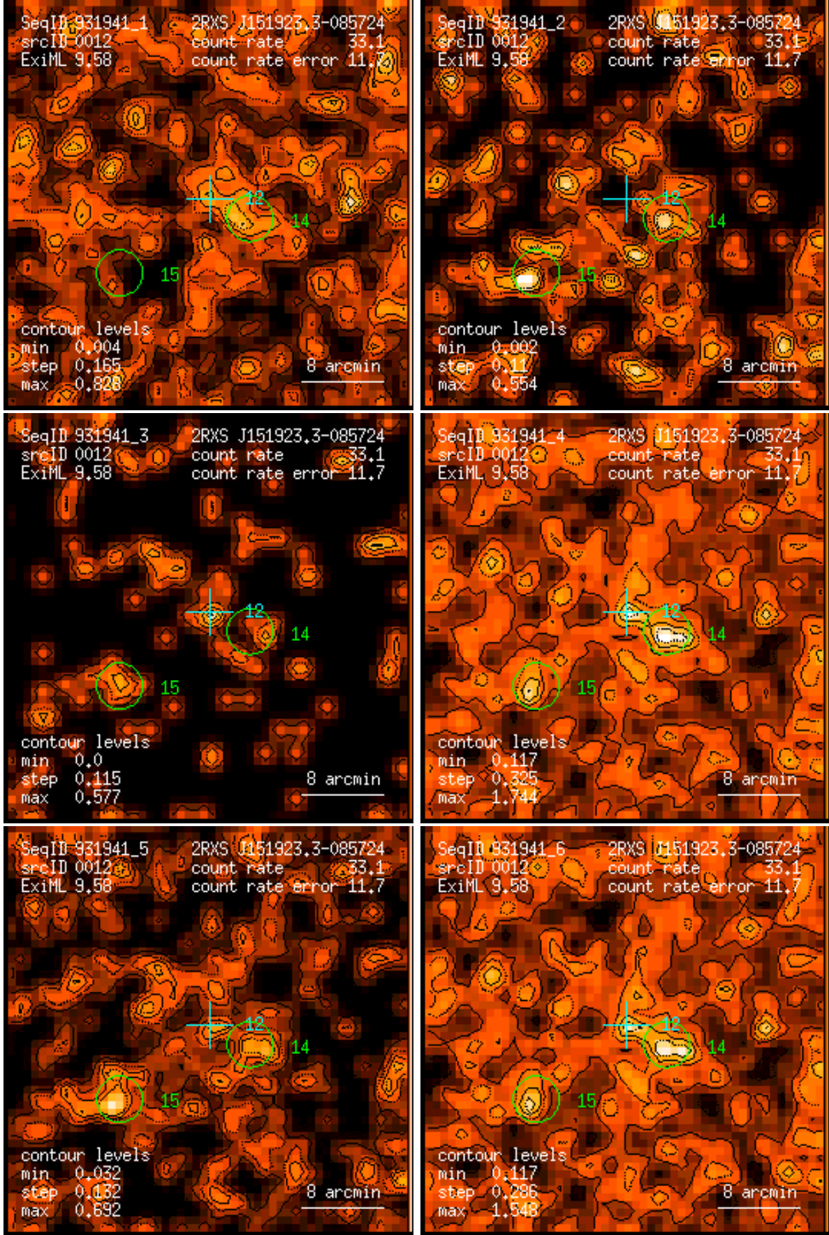
Figure 12: RASS 931941: detection 0012: band rate images, Gaussian filter: (1) PSPC channels 11 – 41, (2) 52 – 90, (3) 91 – 201, (4) 11 – 235, (5) 52 – 201, (6) 11 – 201. Broad band rates in counts/ks. Band rate contour levels in counts/ks/arcmin 2 .
