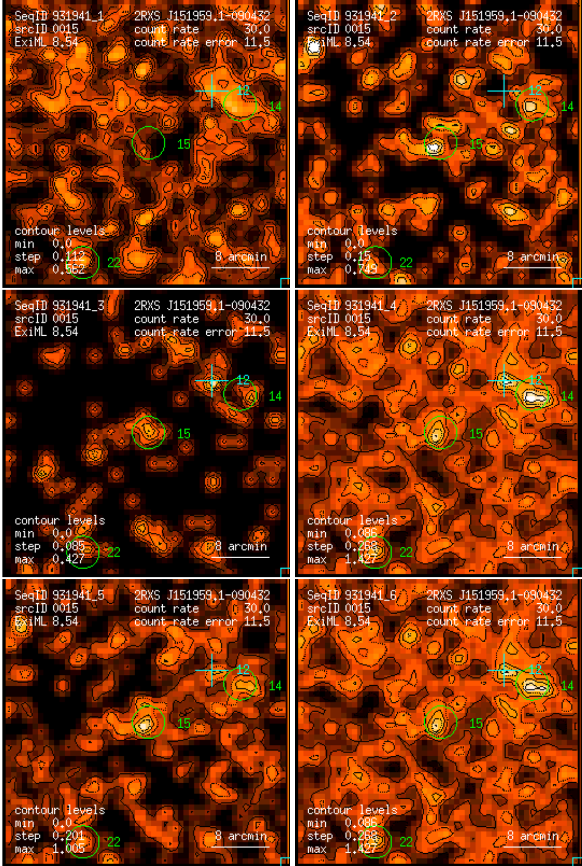
Figure 15: RASS 931941: detection 0015: band rate images, Gaussian filter: (1) PSPC channels 11 – 41, (2) 52 – 90, (3) 91 – 201, (4) 11 – 235, (5) 52 – 201, (6) 11 – 201. Broad band rates in counts/ks. Band rate contour levels in counts/ks/arcmin 2 .
