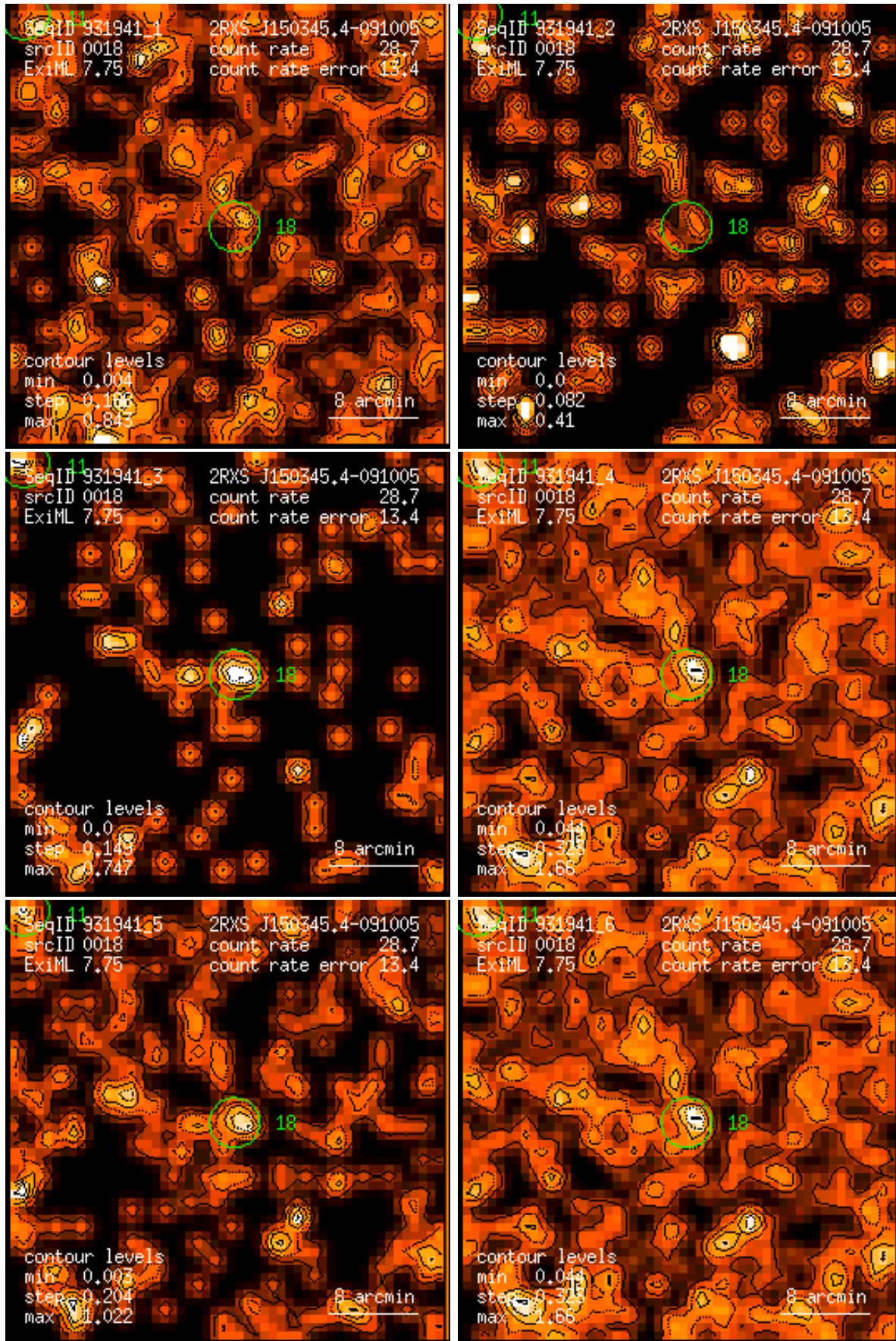
Figure 18: RASS 931941: detection 0018: band rate images, Gaussian filter: (1) PSPC channels 11 – 41, (2) 52 – 90, (3) 91 – 201, (4) 11 – 235, (5) 52 – 201, (6) 11 – 201. Broad band rates in counts/ks. Band rate contour levels in counts/ks/arcmin 2 .
