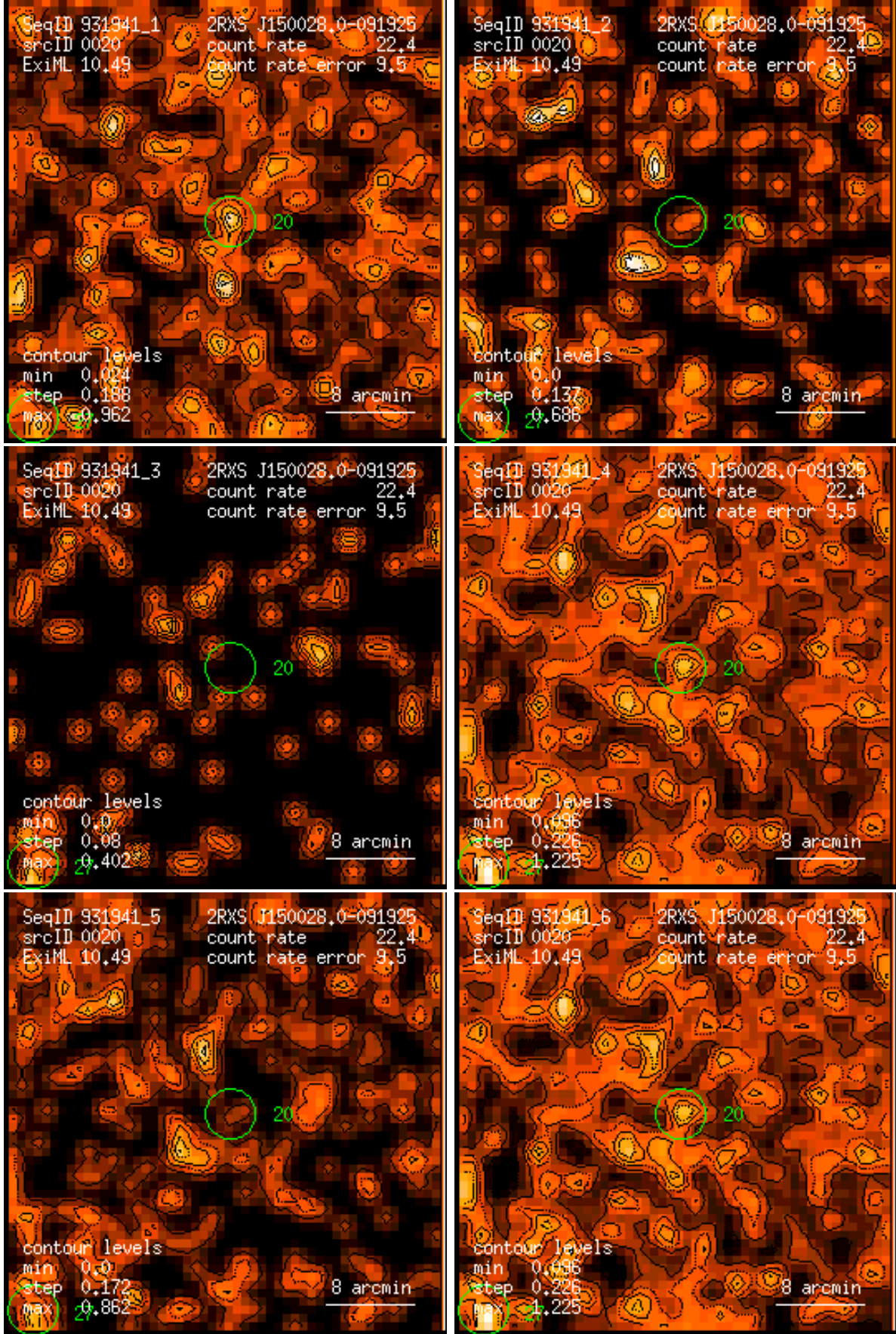
Figure 20: RASS 931941: detection 0020: band rate images, Gaussian filter: (1) PSPC channels 11 – 41, (2) 52 – 90, (3) 91 – 201, (4) 11 – 235, (5) 52 – 201, (6) 11 – 201. Broad band rates in counts/ks. Band rate contour levels in counts/ks/arcmin 2 .
