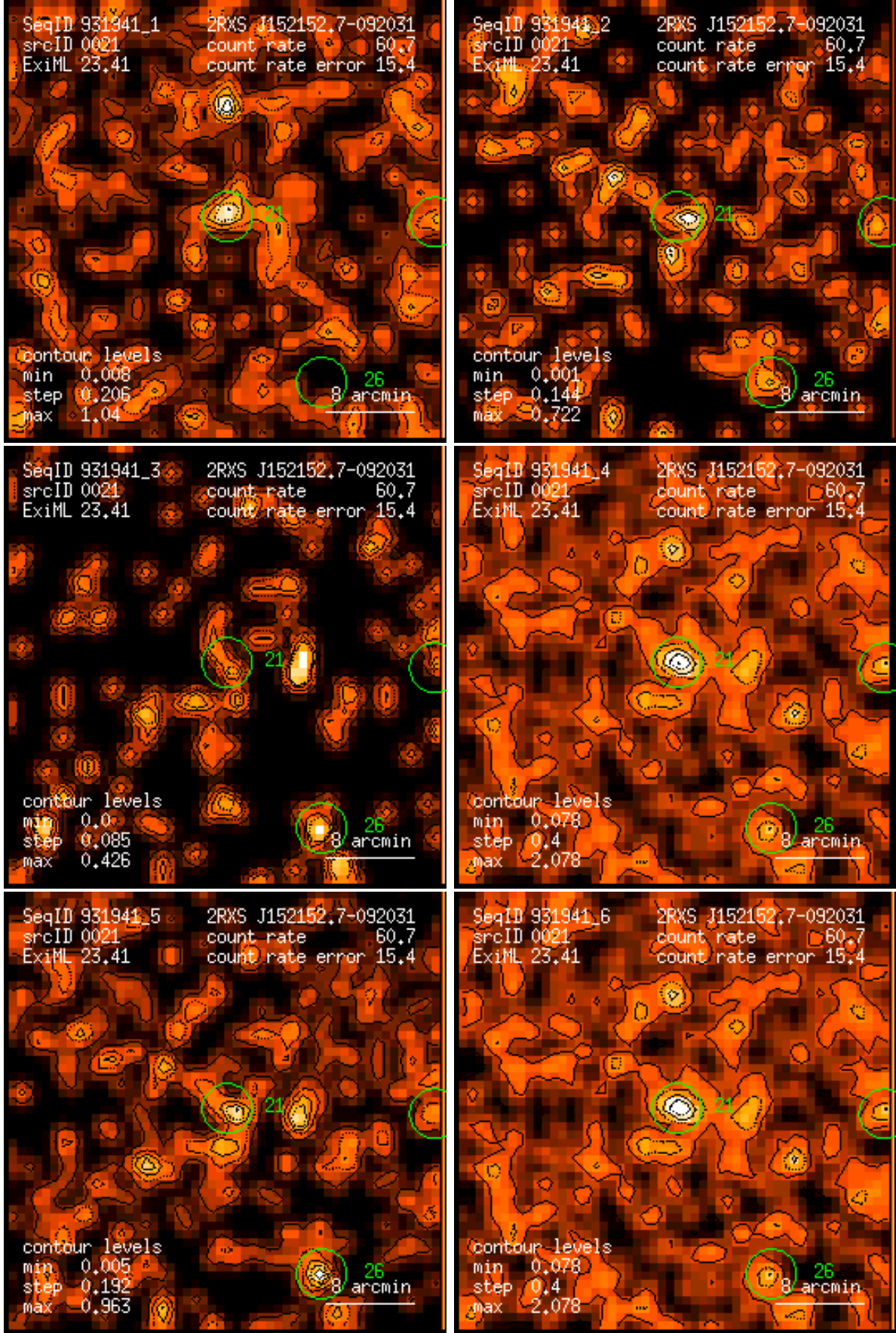
Figure 21: RASS 931941: detection 0021: band rate images, Gaussian filter: (1) PSPC channels 11 – 41, (2) 52 – 90, (3) 91 – 201, (4) 11 – 235, (5) 52 – 201, (6) 11 – 201. Broad band rates in counts/ks. Band rate contour levels in counts/ks/arcmin 2 .
