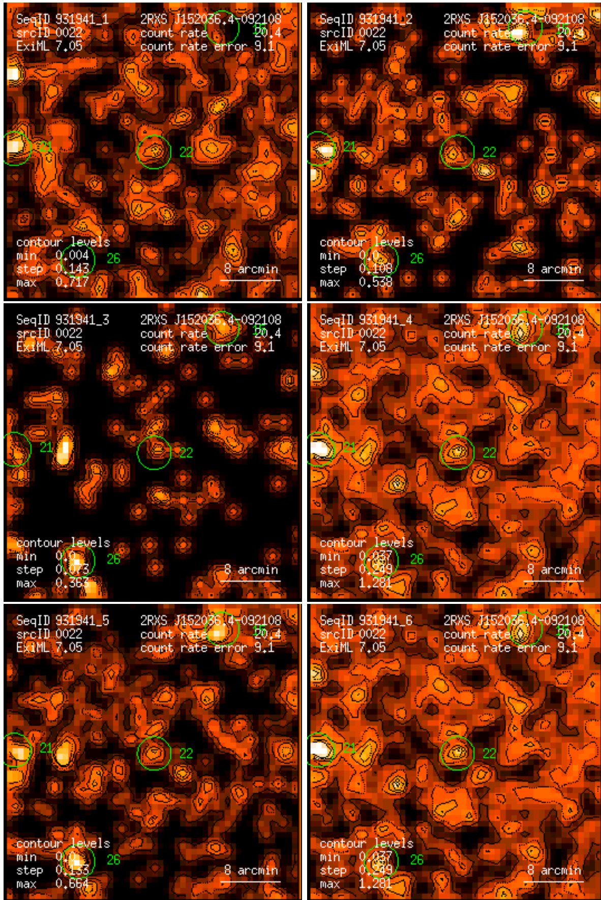
Figure 22: RASS 931941: detection 0022: band rate images, Gaussian filter: (1) PSPC channels 11 – 41, (2) 52 – 90, (3) 91 – 201, (4) 11 – 235, (5) 52 – 201, (6) 11 – 201. Broad band rates in counts/ks. Band rate contour levels in counts/ks/arcmin 2 .
