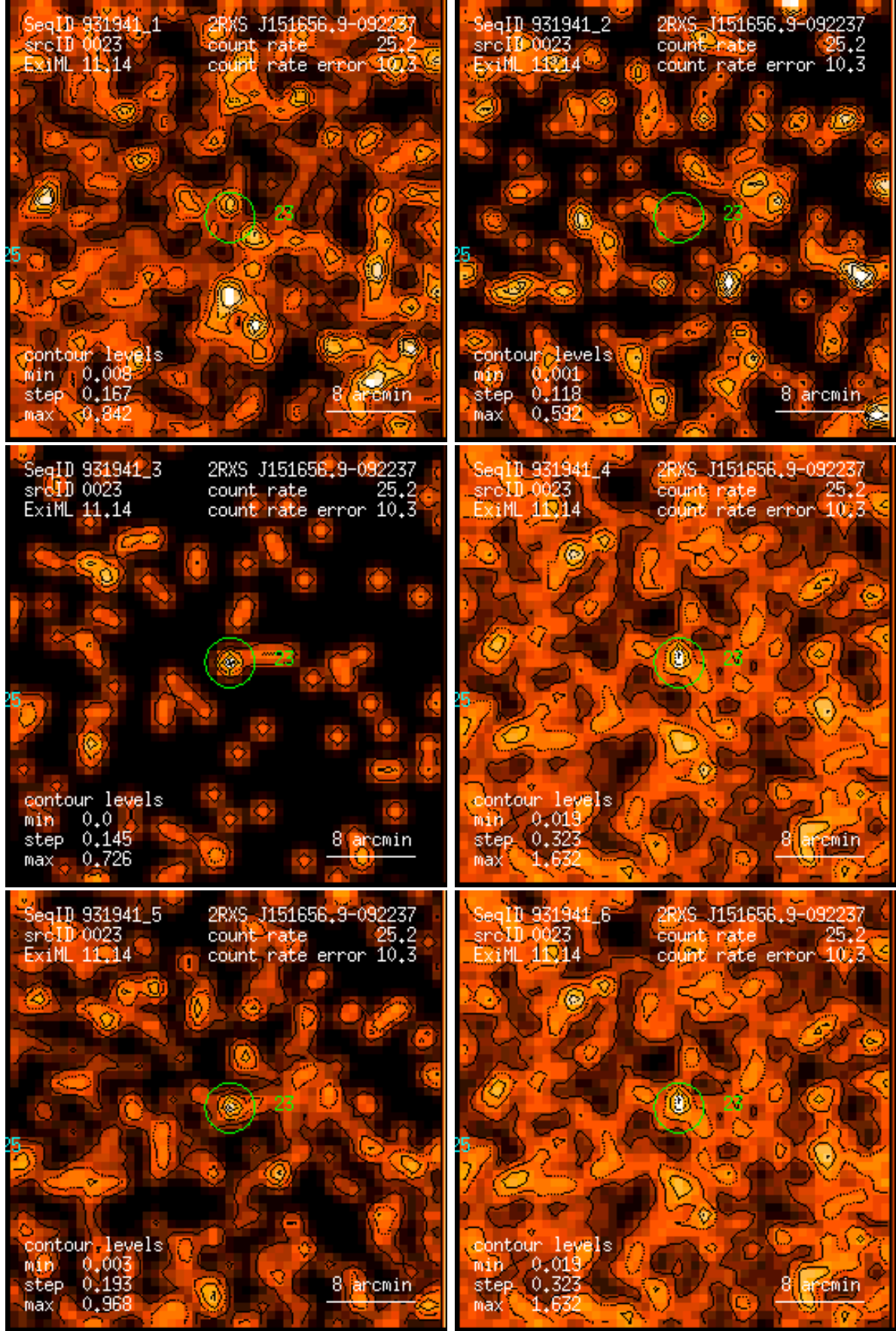
Figure 23: RASS 931941: detection 0023: band rate images, Gaussian filter: (1) PSPC channels 11 – 41, (2) 52 – 90, (3) 91 – 201, (4) 11 – 235, (5) 52 – 201, (6) 11 – 201. Broad band rates in counts/ks. Band rate contour levels in counts/ks/arcmin 2 .
