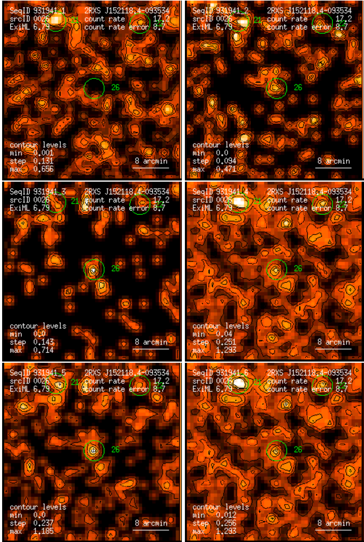
Figure 26: RASS 931941: detection 0026: band rate images, Gaussian filter: (1) PSPC channels 11 – 41, (2) 52 – 90, (3) 91 – 201, (4) 11 – 235, (5) 52 – 201, (6) 11 – 201. Broad band rates in counts/ks. Band rate contour levels in counts/ks/arcmin 2 .
