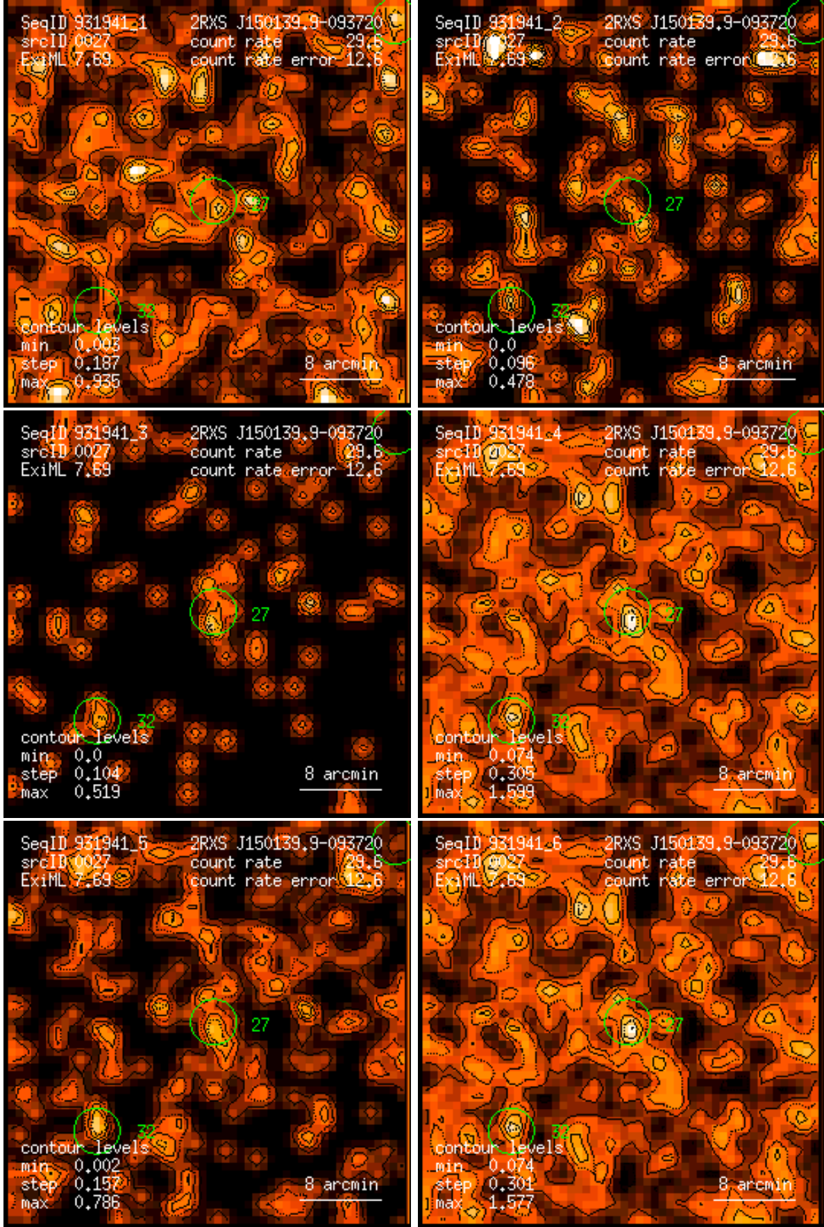
Figure 27: RASS 931941: detection 0027: band rate images, Gaussian filter: (1) PSPC channels 11 – 41, (2) 52 – 90, (3) 91 – 201, (4) 11 – 235, (5) 52 – 201, (6) 11 – 201. Broad band rates in counts/ks. Band rate contour levels in counts/ks/arcmin 2 .
