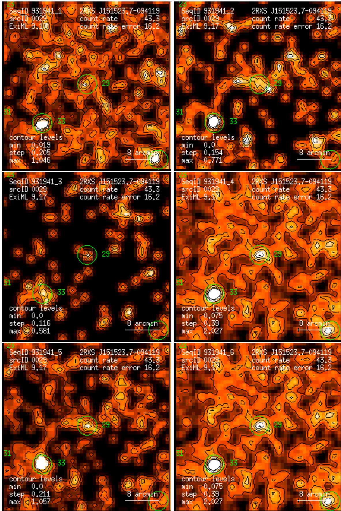
Figure 29: RASS 931941: detection 0029: band rate images, Gaussian filter: (1) PSPC channels 11 – 41, (2) 52 – 90, (3) 91 – 201, (4) 11 – 235, (5) 52 – 201, (6) 11 – 201. Broad band rates in counts/ks. Band rate contour levels in counts/ks/arcmin 2 .
