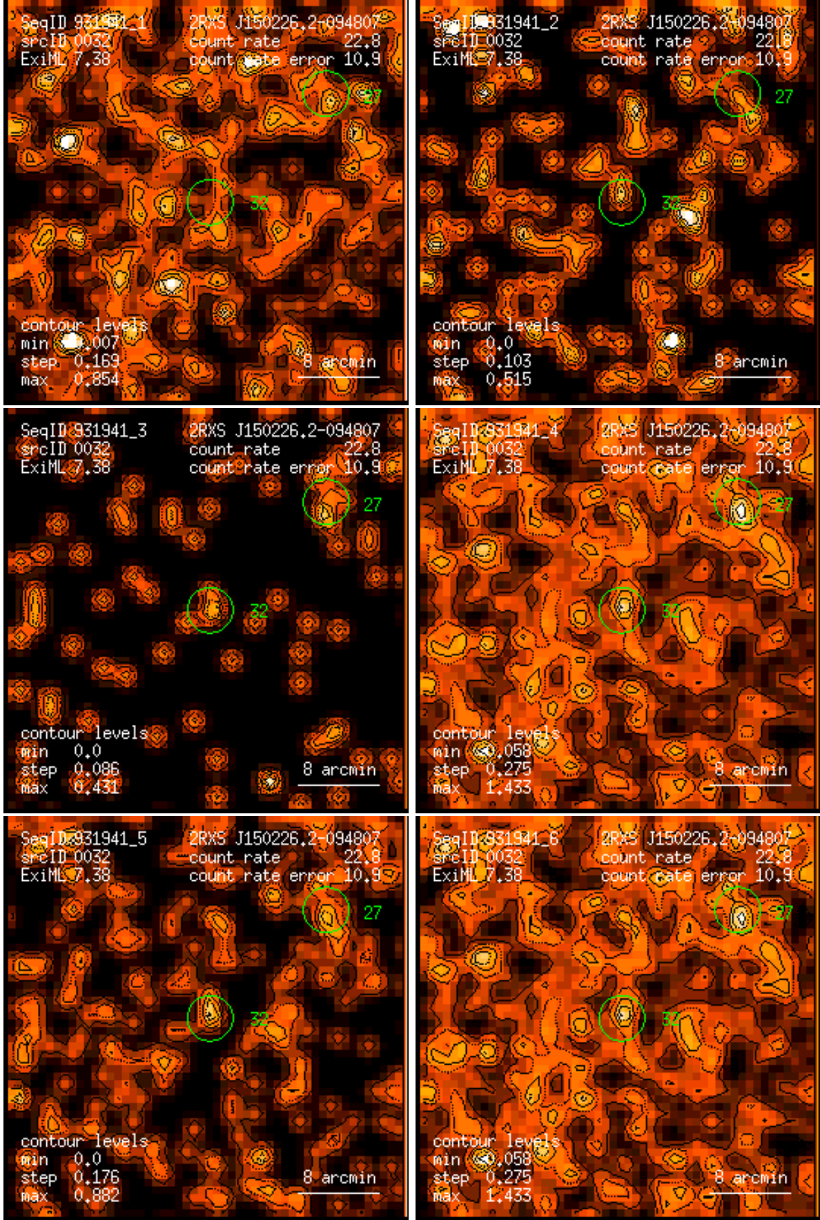
Figure 32: RASS 931941: detection 0032: band rate images, Gaussian filter: (1) PSPC channels 11 – 41, (2) 52 – 90, (3) 91 – 201, (4) 11 – 235, (5) 52 – 201, (6) 11 – 201. Broad band rates in counts/ks. Band rate contour levels in counts/ks/arcmin 2 .
