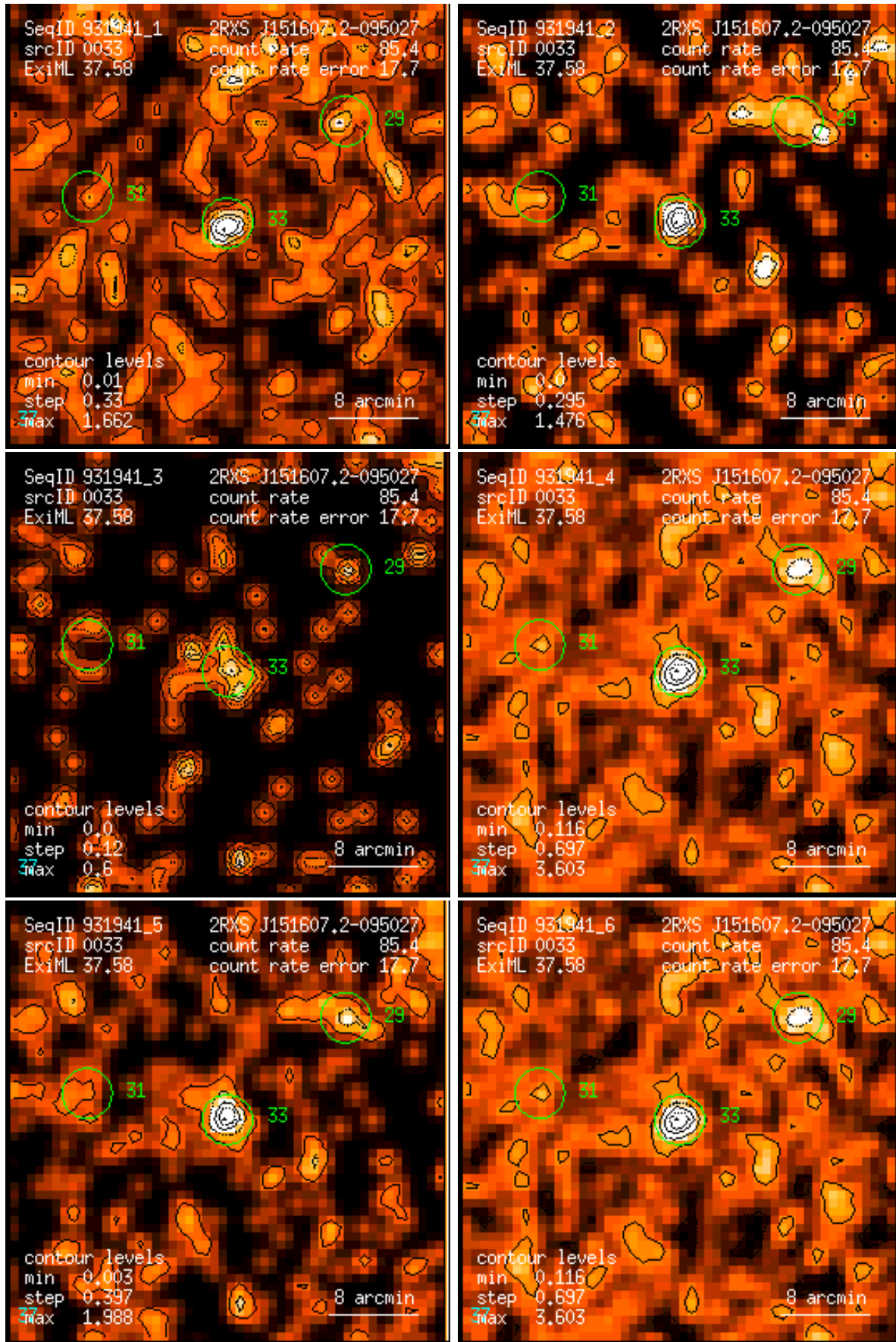
Figure 33: RASS 931941: detection 0033: band rate images, Gaussian filter: (1) PSPC channels 11 – 41, (2) 52 – 90, (3) 91 – 201, (4) 11 – 235, (5) 52 – 201, (6) 11 – 201. Broad band rates in counts/ks. Band rate contour levels in counts/ks/arcmin 2 .
