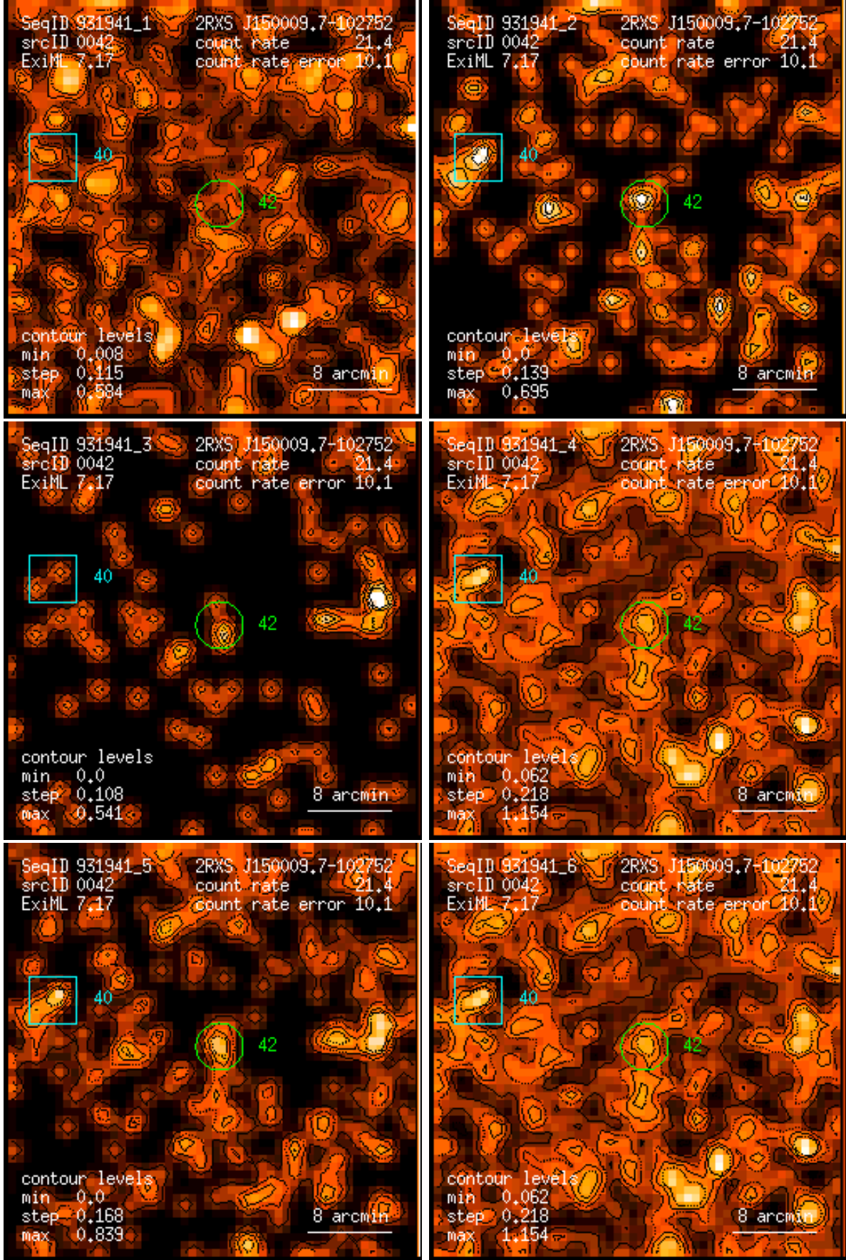
Figure 42: RASS 931941: detection 0042: band rate images, Gaussian filter: (1) PSPC channels 11 – 41, (2) 52 – 90, (3) 91 – 201, (4) 11 – 235, (5) 52 – 201, (6) 11 – 201. Broad band rates in counts/ks. Band rate contour levels in counts/ks/arcmin 2 .
