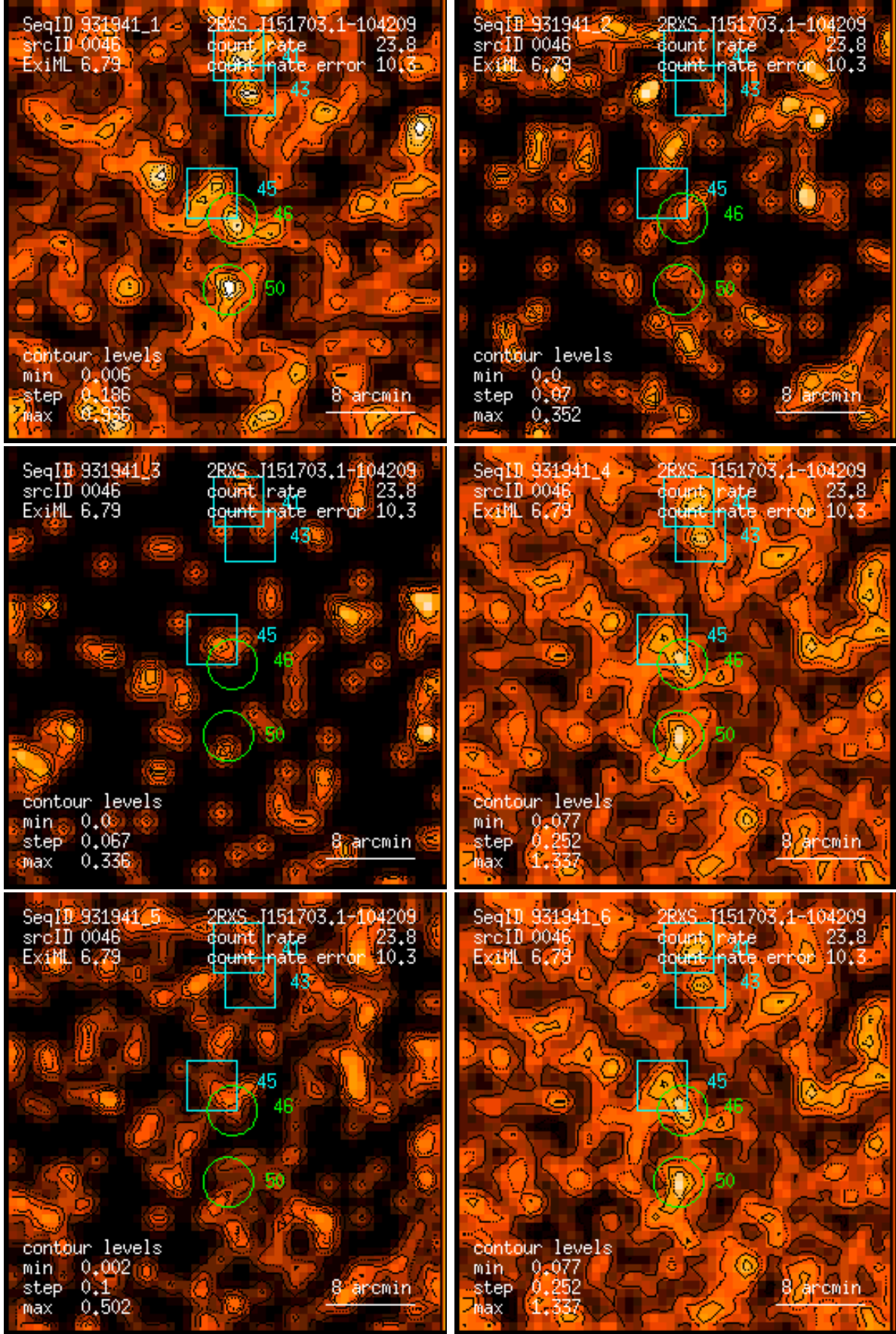
Figure 46: RASS 931941: detection 0046: band rate images, Gaussian filter: (1) PSPC channels 11 – 41, (2) 52 – 90, (3) 91 – 201, (4) 11 – 235, (5) 52 – 201, (6) 11 – 201. Broad band rates in counts/ks. Band rate contour levels in counts/ks/arcmin 2 .
