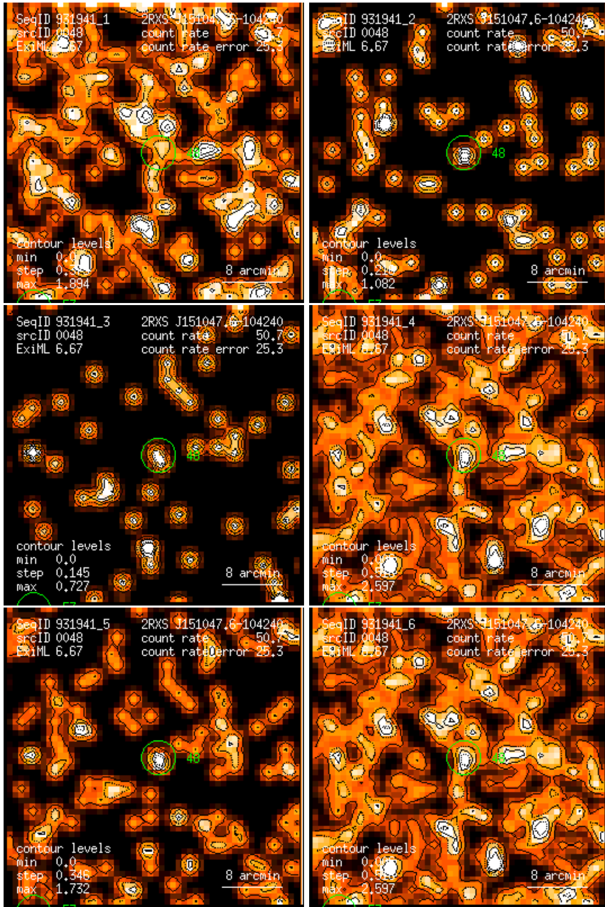
Figure 48: RASS 931941: detection 0048: band rate images, Gaussian filter: (1) PSPC channels 11 – 41, (2) 52 – 90, (3) 91 – 201, (4) 11 – 235, (5) 52 – 201, (6) 11 – 201. Broad band rates in counts/ks. Band rate contour levels in counts/ks/arcmin 2 .
