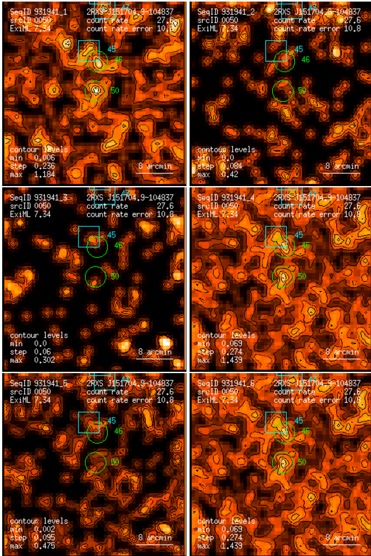
Figure 50: RASS 931941: detection 0050: band rate images, Gaussian filter: (1) PSPC channels 11 – 41, (2) 52 – 90, (3) 91 – 201, (4) 11 – 235, (5) 52 – 201, (6) 11 – 201. Broad band rates in counts/ks. Band rate contour levels in counts/ks/arcmin 2 .
