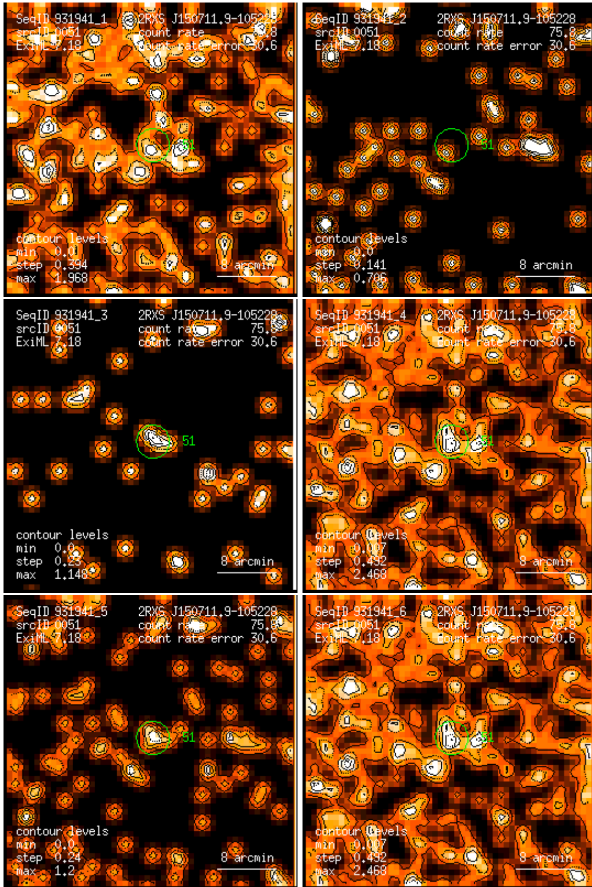
Figure 51: RASS 931941: detection 0051: band rate images, Gaussian filter: (1) PSPC channels 11 – 41, (2) 52 – 90, (3) 91 – 201, (4) 11 – 235, (5) 52 – 201, (6) 11 – 201. Broad band rates in counts/ks. Band rate contour levels in counts/ks/arcmin 2 .
