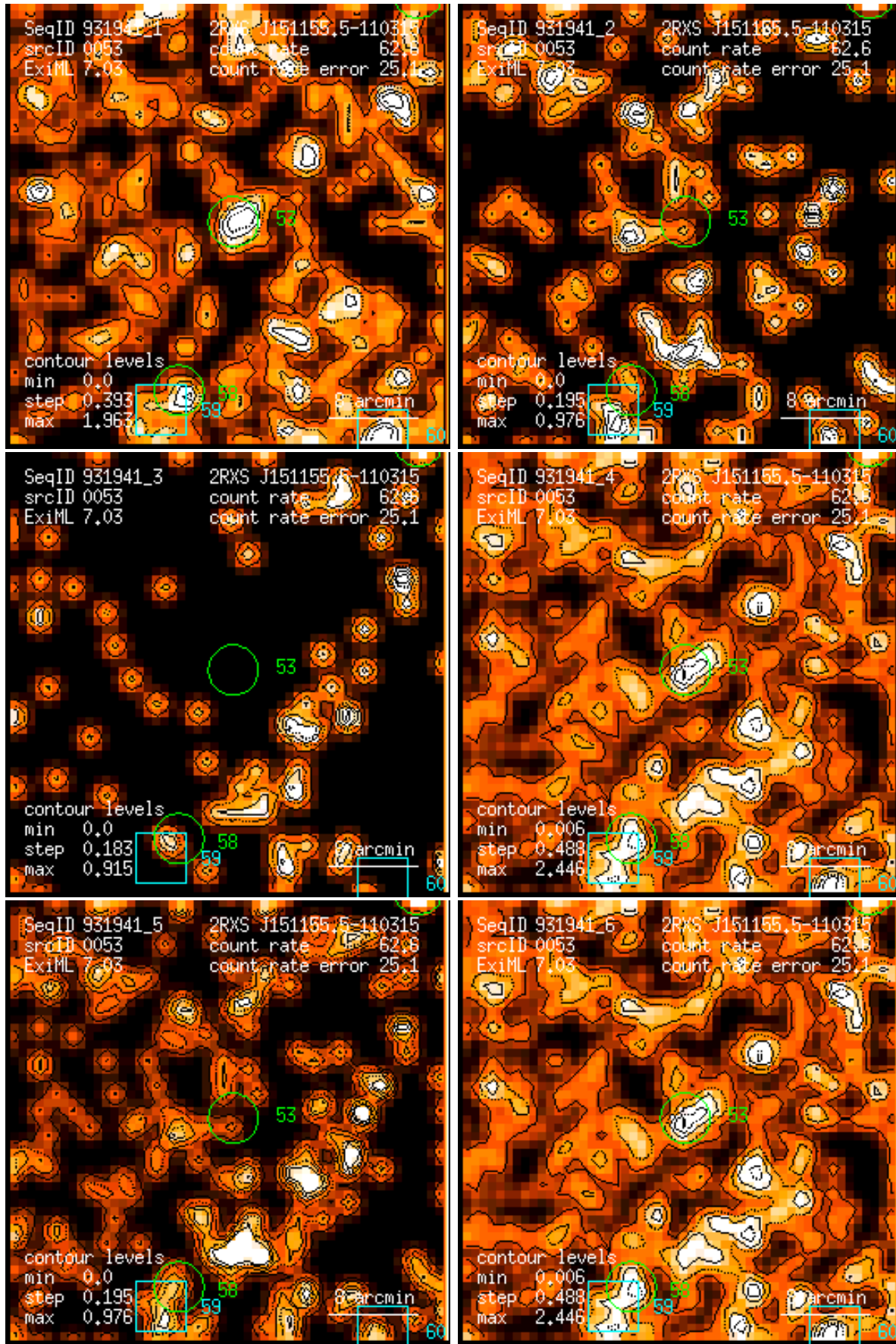
Figure 53: RASS 931941: detection 0053: band rate images, Gaussian filter: (1) PSPC channels 11 – 41, (2) 52 – 90, (3) 91 – 201, (4) 11 – 235, (5) 52 – 201, (6) 11 – 201. Broad band rates in counts/ks. Band rate contour levels in counts/ks/arcmin 2 .
