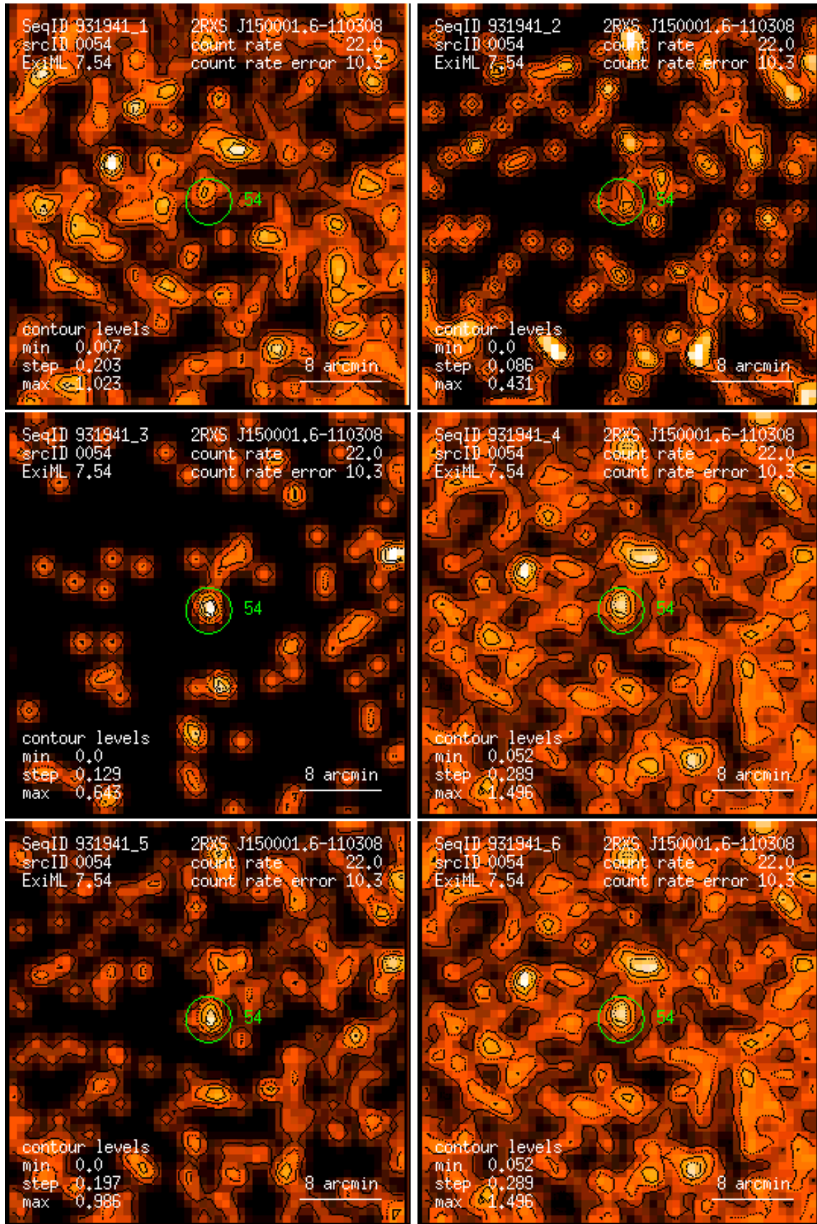
Figure 54: RASS 931941: detection 0054: band rate images, Gaussian filter: (1) PSPC channels 11 – 41, (2) 52 – 90, (3) 91 – 201, (4) 11 – 235, (5) 52 – 201, (6) 11 – 201. Broad band rates in counts/ks. Band rate contour levels in counts/ks/arcmin 2 .
