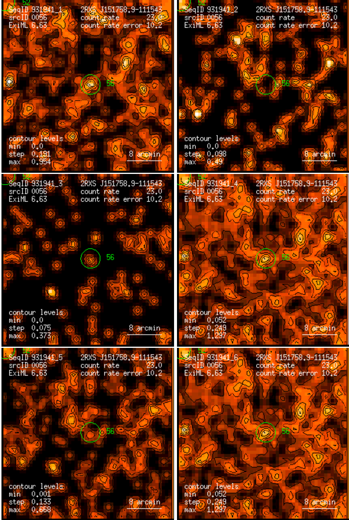
Figure 56: RASS 931941: detection 0056: band rate images, Gaussian filter: (1) PSPC channels 11 – 41, (2) 52 – 90, (3) 91 – 201, (4) 11 – 235, (5) 52 – 201, (6) 11 – 201. Broad band rates in counts/ks. Band rate contour levels in counts/ks/arcmin 2 .
