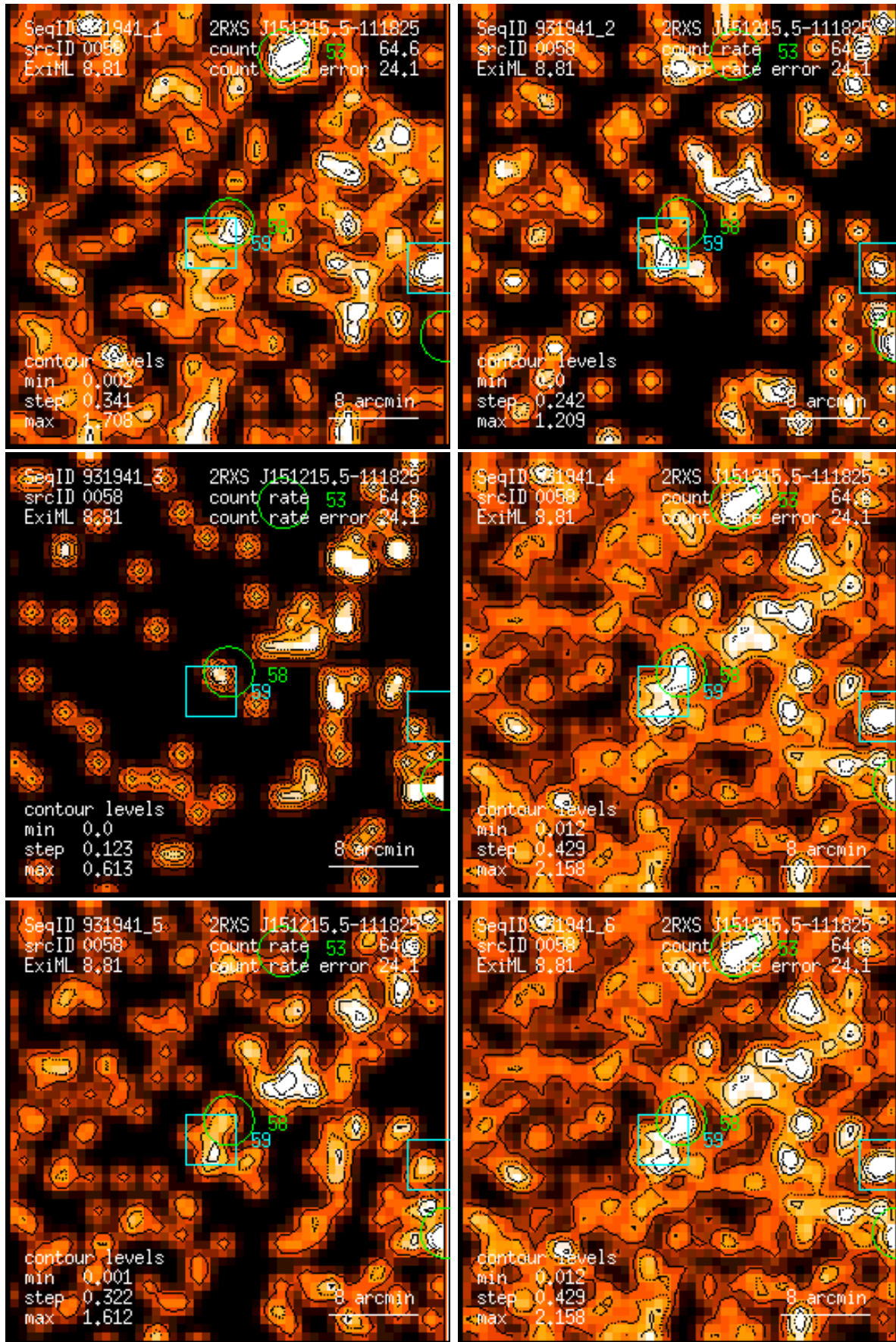
Figure 58: RASS 931941: detection 0058: band rate images, Gaussian filter: (1) PSPC channels 11 – 41, (2) 52 – 90, (3) 91 – 201, (4) 11 – 235, (5) 52 – 201, (6) 11 – 201. Broad band rates in counts/ks. Band rate contour levels in counts/ks/arcmin 2 .
